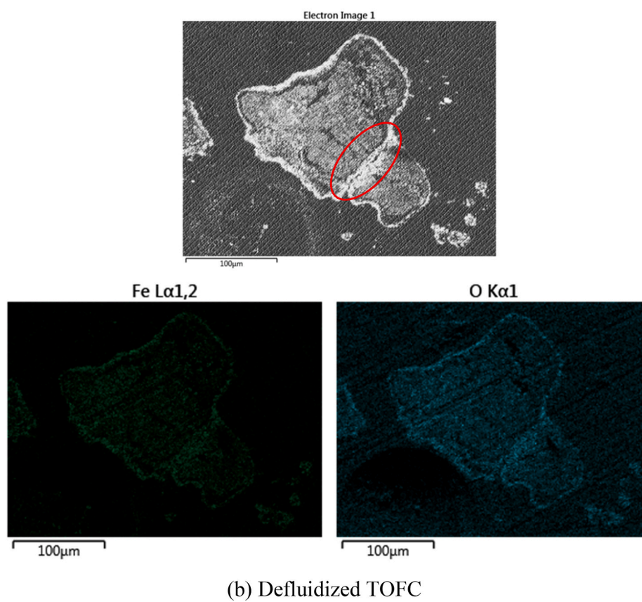
Fig. 10. The elemental distribution of iron (Fe) and oxygen (O) in TOFC particles. The red circle indicates the surface joint between particles.
