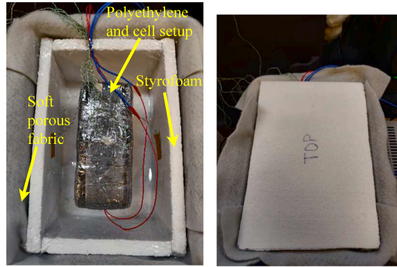
(c) Experimental setup of the cell and polyethylene placed in with the Styrofoam lid. (d) The experimental setup the Styrofoam box.
