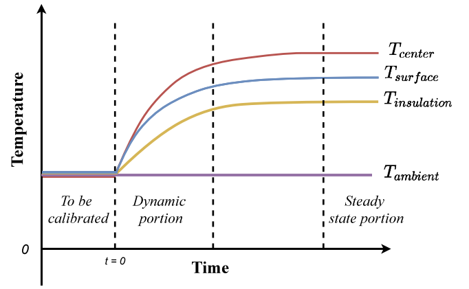
Fig. 3. Test for finding C_{p_{out}} and R_{cell} .
