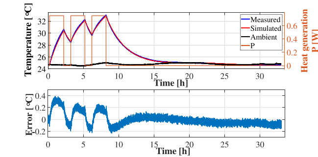
(c) Comparison between the measured and the modelled surface temperature. C_{p_{cell}} = 1037.56 \text{ JK}^{-1}\text{kg}^{-1} and R_{cell} = 0.76 \text{ KW}^{-1} are used in the model.
