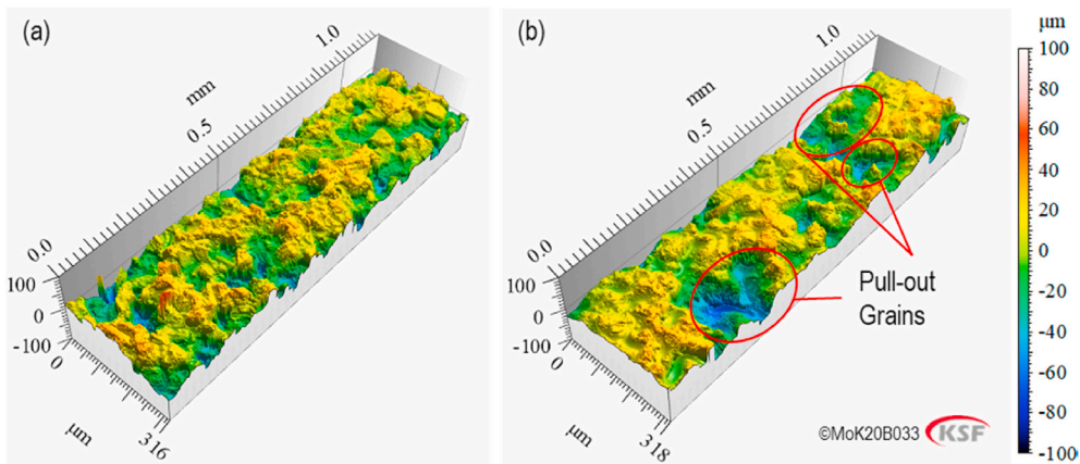
Fig. 14. The micro-topography of the wheel with a) concentration of 150 and b) concentration of 200 after grinding process with v_c = 10 m/s, a_e = 6 \mu\text{m} , v_w = 480 mm/min, and \text{Aggr.} \approx 44 .
