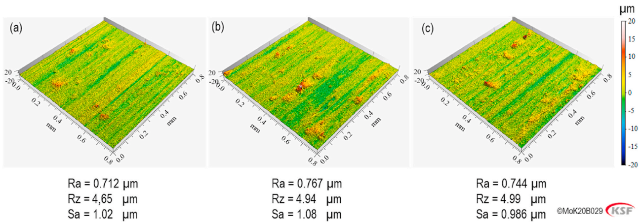
Fig. 12. Surface topography of the workpiece after micro-grinding process for a) conventional part, b) AM BD 20, and c) AM BD 30 ( v_c = 10 m/s, a_e = 10 \mu\text{m} , v_w = 800 mm/min, and \text{Aggr.} \approx 100 ).
