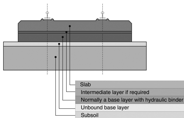
Figure 2. Typical section through slab track supported on terrain (source: Institute of Road, Railway and Airfield Construction, Technical University of Munich, Fiedler)
