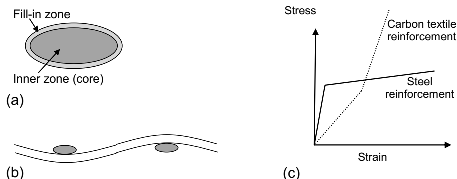
Figure 5. (a) Conceptual figure of a yarn, based on (Hartig, J., 2008). (b) Yarns running in waves above and below transverse yarns. Schematic, based on (Brameshuber, 2006). (c) Idealized stress versus strain for a carbon textile reinforcement compared to traditional steel reinforcement. From (Schladitz et al. , 2012).
