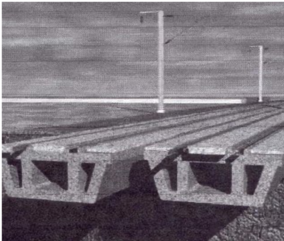
Figure 7. Deck Track System – A 200 m test section of the track constructed in 1999 near Rotterdam, the Netherlands (Bos, J. and Stuit, 1999).
