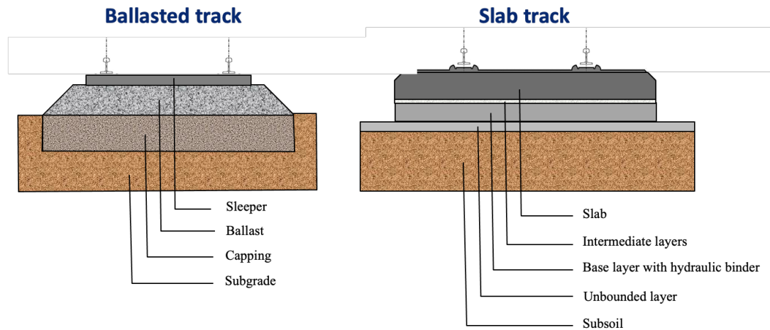
Figure 1. Schematic illustration of Ballasted track and slab track foundation
