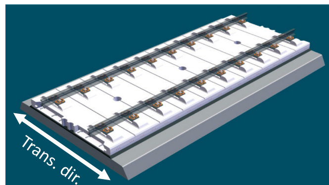
Figure 8. Prefabricated track system Bögl.
