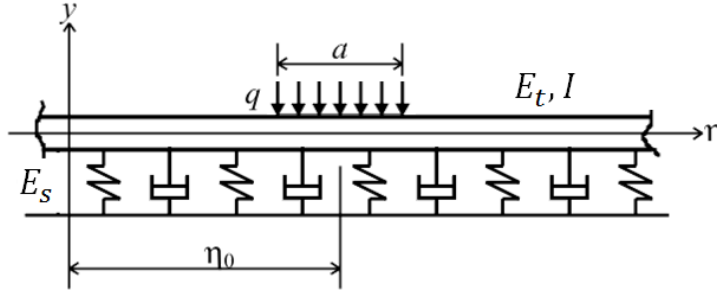
Figure 4. Schematic representation of a beam on damped elastic foundation under line load (Akbarian, 2012).
