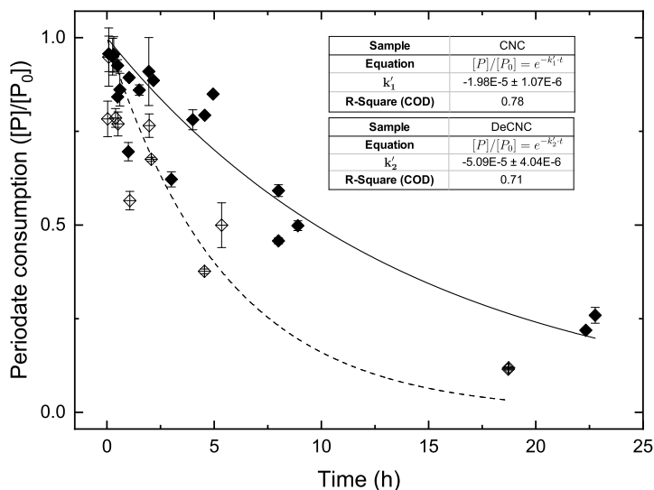
Fig. 2: Consumption of periodate during the oxidation of the CNCs (◆) and desulfCNCs (◇). The equations containing k_1' and k_2' correspond to CNC and desulfCNC, respectively. R-square, i.e. , the coefficient of determination (COD), qualifies the regression. These curves are comprised of three oxidation series for each CNC derivative. Selected points are excluded for clarity but are included in the fitting and statistical analysis.
