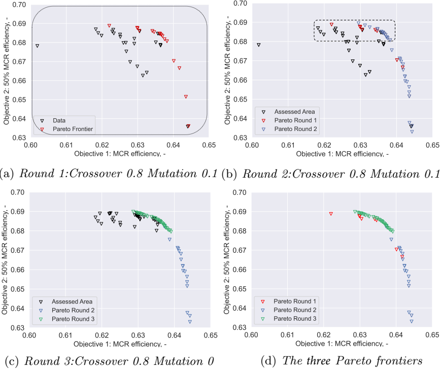
Figure 5.5: Evolution of optimisation algorithm with two interactive steps
