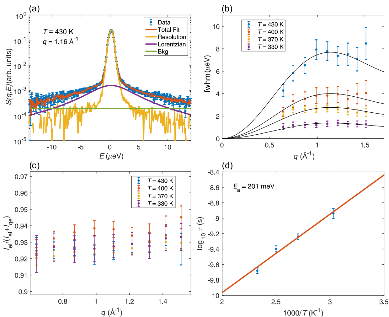
Figure 3. QENS data of SrVO 2 H from neutron backscattering spectroscopy measured on HFBS. (a) Example fitting to the quasi-elastic line shape of SrVO 2 H for T = 430\text{ K} and q = 1.16\text{ \AA}^{-1} . (b) fwhm of the quasi-elastic component as a function of T and q together with fits to the Chudley–Elliott model describing long-range jump diffusion (solid black lines). (c) Fraction of elastic scattering as a function of T and q . (d) Fit to an Arrhenius law of the extracted mean residence time \tau .
