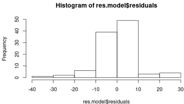
Figure 6.6: A histogram of the residuals
