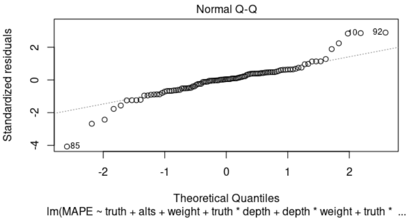
Figure 6.8: The normal quantile-quantile plot
