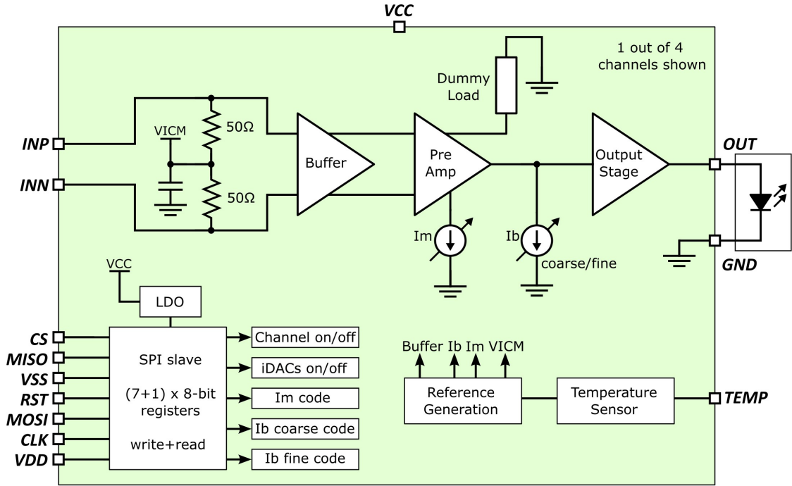
Figure 6.5: Schematic block diagram of a single channel of the VCSEL Driver.
