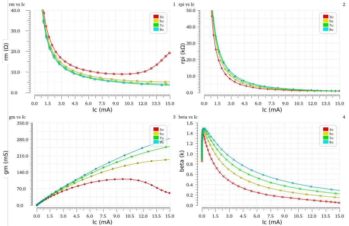
Figure 3.3: Simulated SiGe HBT small signal parameters vs collector current for various emitter sizes.
