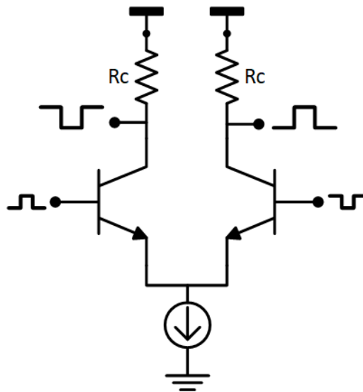
Figure 3.2: Differential CE amplifier.
