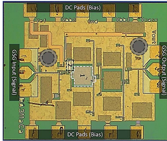
Figure 4.7: Microphoto of the M-SSDA. Region 1 (enclosed by white dashed lines) marks the location of the inter-stage capacitor C_{BLOCK} between tier 1 and tier 2, and the associated vias and metal connections; region 2 (enclosed by black dashed lines) marks the location of peaking inductances L_{ce} and L_{cc} . Dashed circles indicate location of through-substrate vias.
