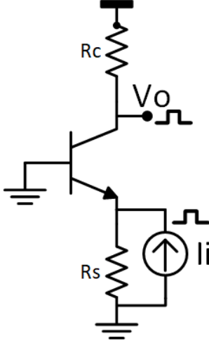
(c) Common Base.
