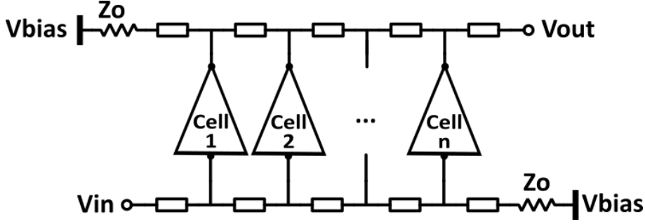
Figure 4.1: Typical topology of a distributed amplifier.
