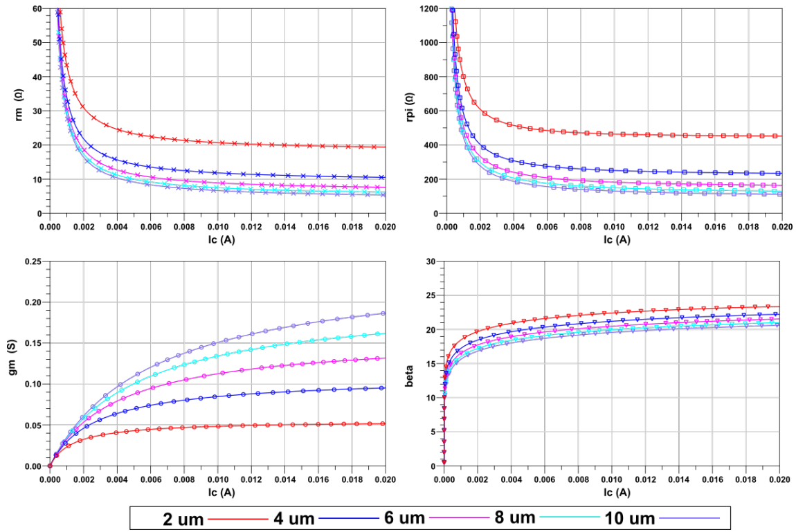
Figure 3.4: Simulated InP 130 nm DHBT small signal parameters vs collector current for various emitter sizes.
