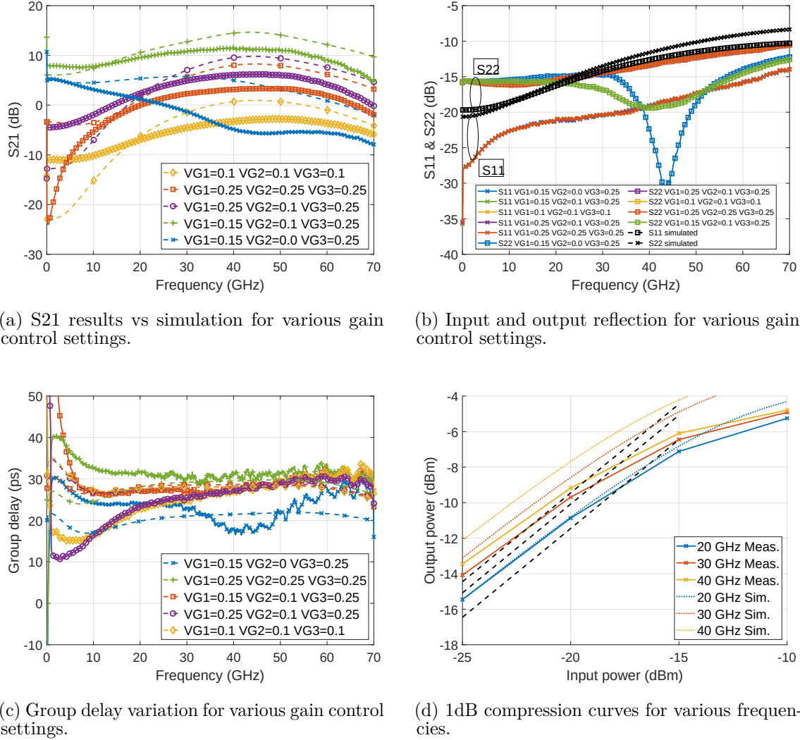
Figure 5.11: Frequency domain measurements of the equalizer MMIC. Tap coefficients VG1, VG2, and VG3 refer to negative voltages.
