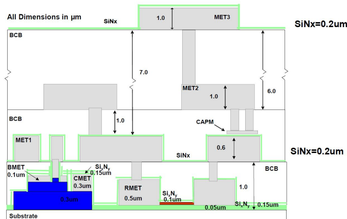
Figure 5.2: Cross-section of the 130 nm InP DHBT process.
