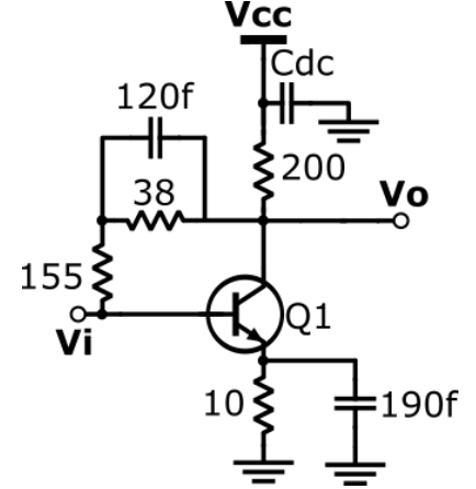
(b) Schematics of the CE TIA.
