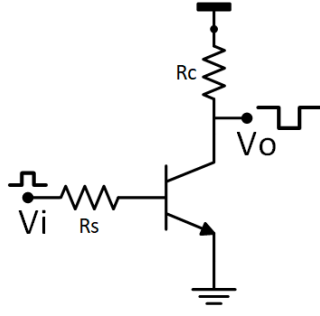
(a) Common Emitter.
