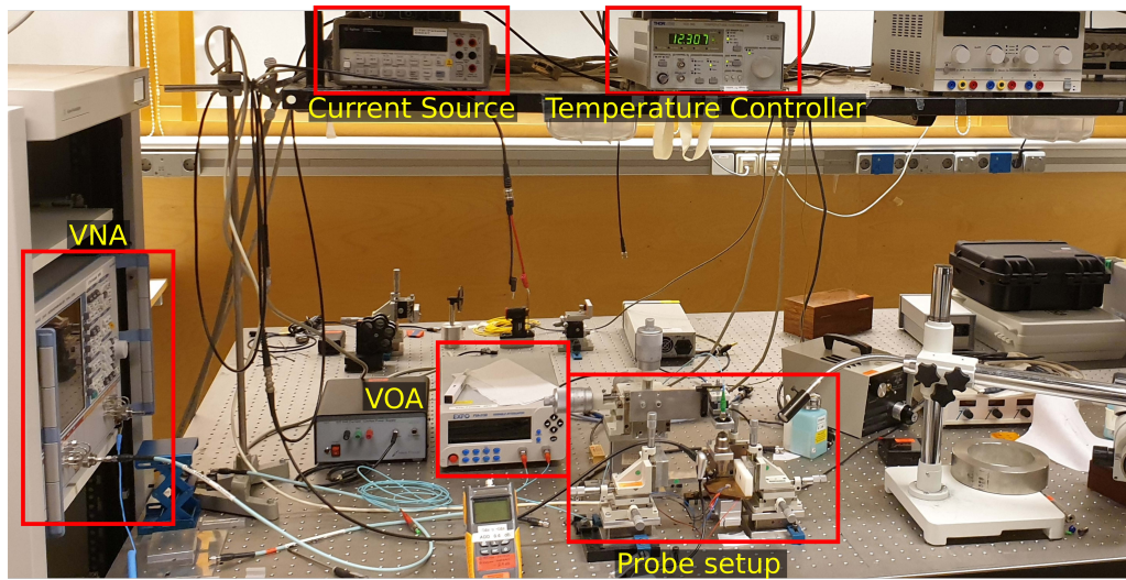
(a) S-parameter measurement setup photo.
