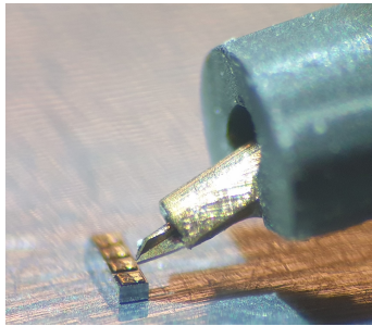
(b) VCSEL array under the probe.
