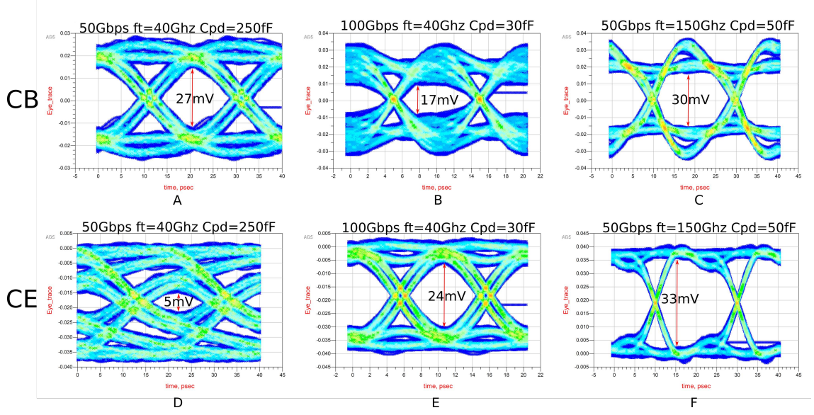
Figure 5.6: Simulated optical time domain eye diagrams for the two TIAs for three photodiode scenarios.
