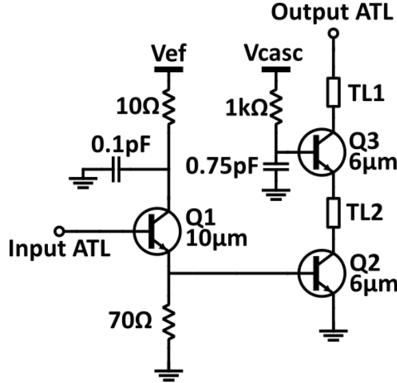
Figure 4.3: Circuit schematic of a single CC-Cascode cell.
