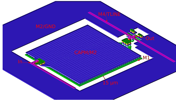
Figure 4.8: Structure and interconnects of the inter-stage ac-coupling capacitors together with the input and output matching transmission lines, used in the E/M simulations.
