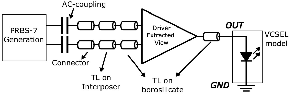
Figure 6.4: Block diagram of the test bench used for the design of the driver.
