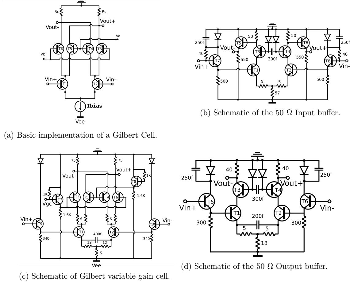
Figure 5.10: Circuit schematics of the a typical Gilbert cell, input buffer, variable gain cell, and output buffer.
