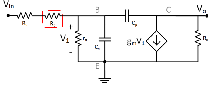
(b) CE small signal high frequency circuit.
