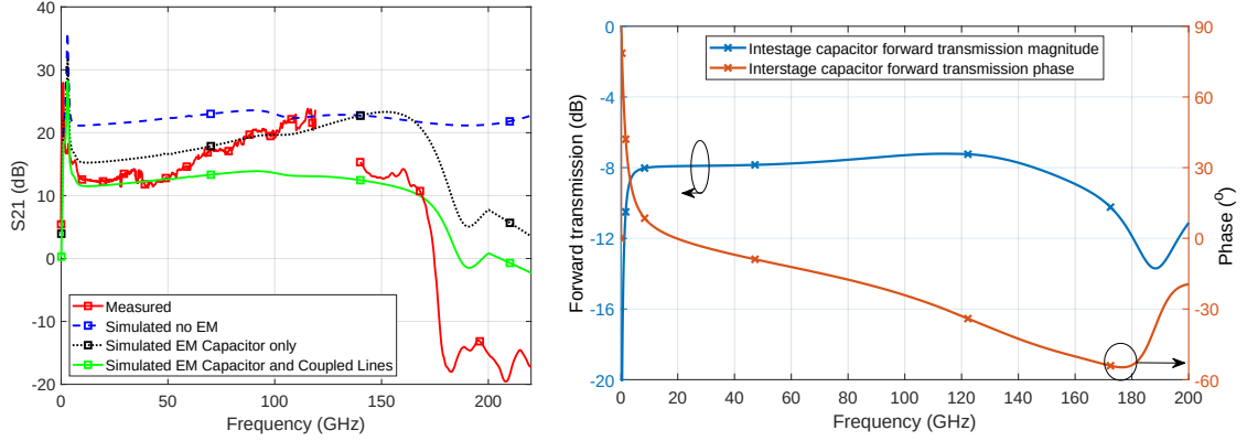
(a) Bandwidth- and gain-limiting effect of inter-stage capacitors and transmission line coupling. (b) Forward transmission simulation of inter-stage Capacitor.
