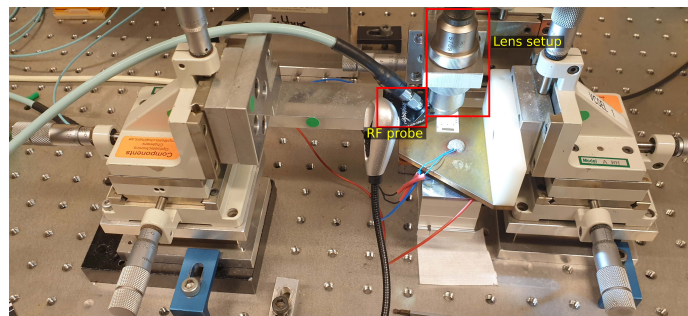
(c) S-parameter probe and lens-coupling setup.
