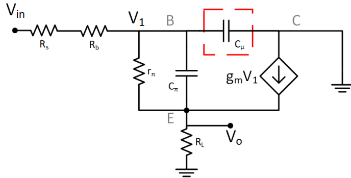
(f) CC small signal high frequency circuit.
