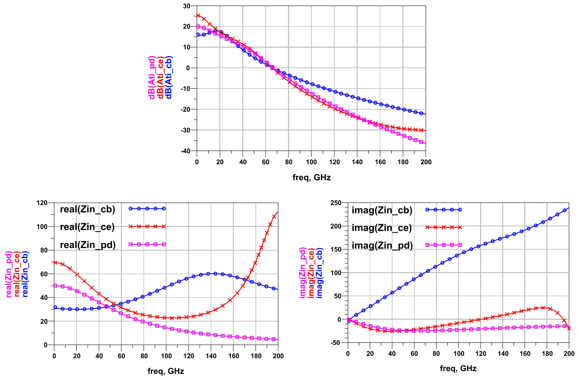
Figure 5.7: Simulated Ti-bandwidth and input impedance of the scenario T1 PD, connected to the CB, CE or a 50 Ohm load.
