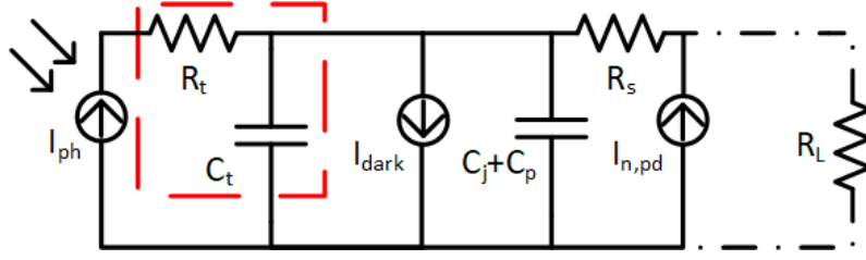
Figure 2.6: PD equivalent model.
