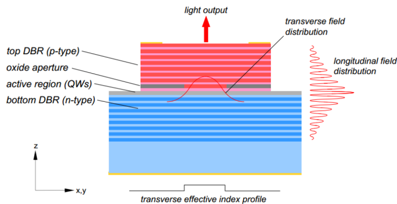
Figure 2.3: Cross-section of a typical VCSEL [18].
