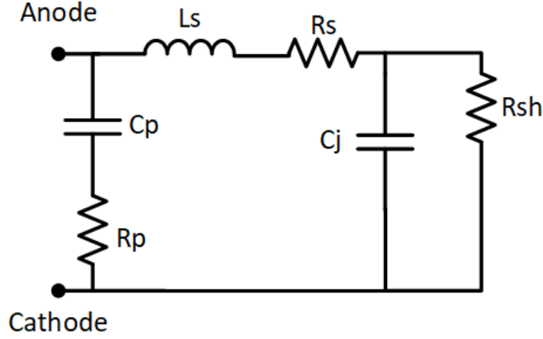
Figure 2.5: PD electrical parasitics model.
