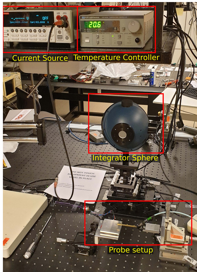
Figure 6.1: Experimental setup for the IPV VCSEL measurements.
