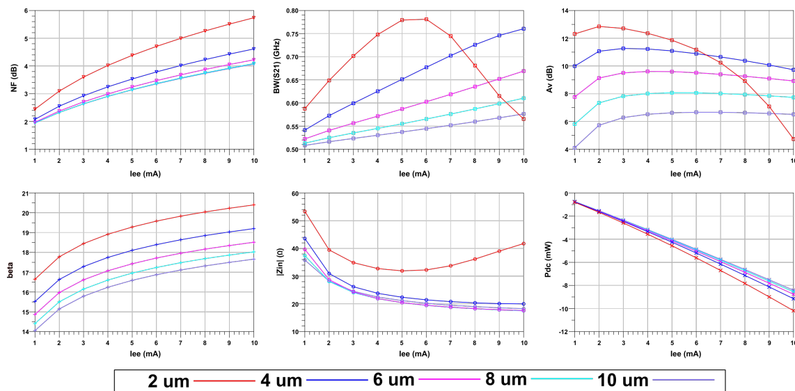
Figure 5.3: Ideal CB amplifier parameters for various emitter sizes as a function of emitter current.
