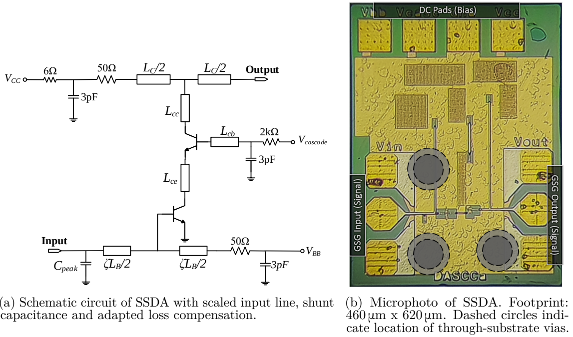
Figure 4.5: SSDA: Circuit diagram and MMIC microphotograph
