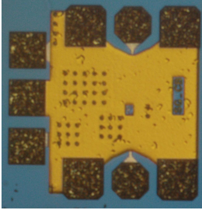
(c) Micrograph of the CB TIA.
