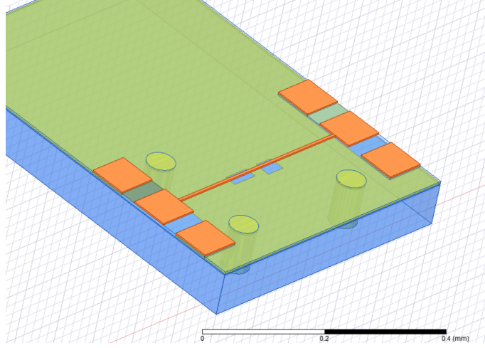
(a) Simplified SSDA model with through transmission line for substrate mode simulation.
