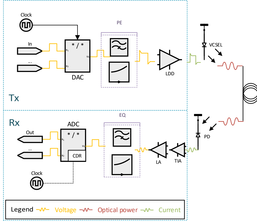
Figure 2.2: Optical link breakdown with the receiver (RX) and transmitter (TX) subsystems assuming heterogeneous integration.
