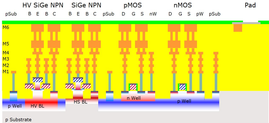
Figure 5.8: Cross-section of the 130 nm SiGe HBT process by Infineon.
