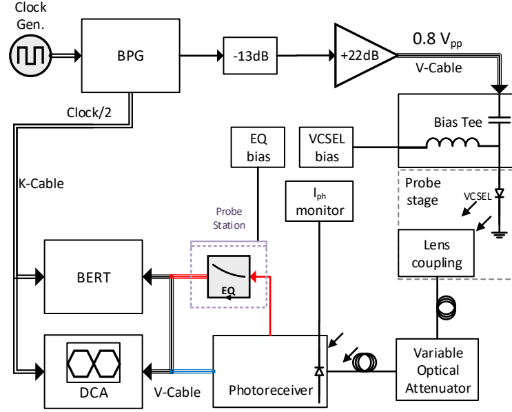
(b) Experimental setup schematics.
