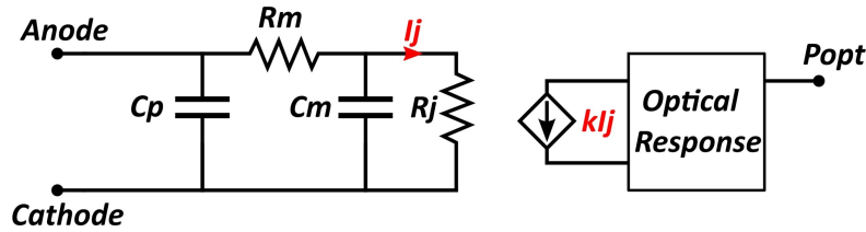
Figure 6.3: VCSEL parasitic model used for fitting.
