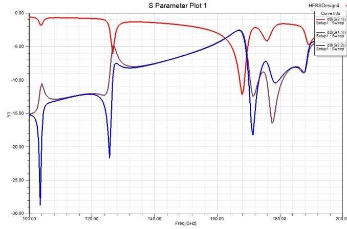
(b) Results of the substrate mode EM simulation.
