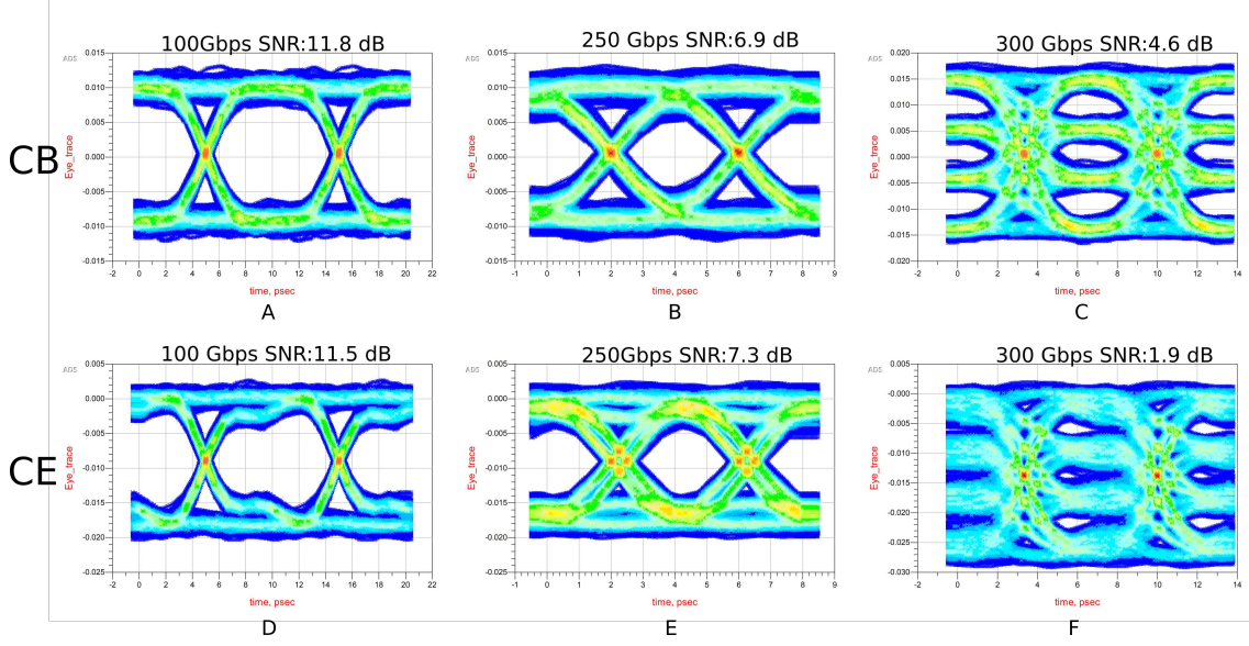
Figure 5.5: Simulated electrical time domain eye diagrams for the two TIAs.
