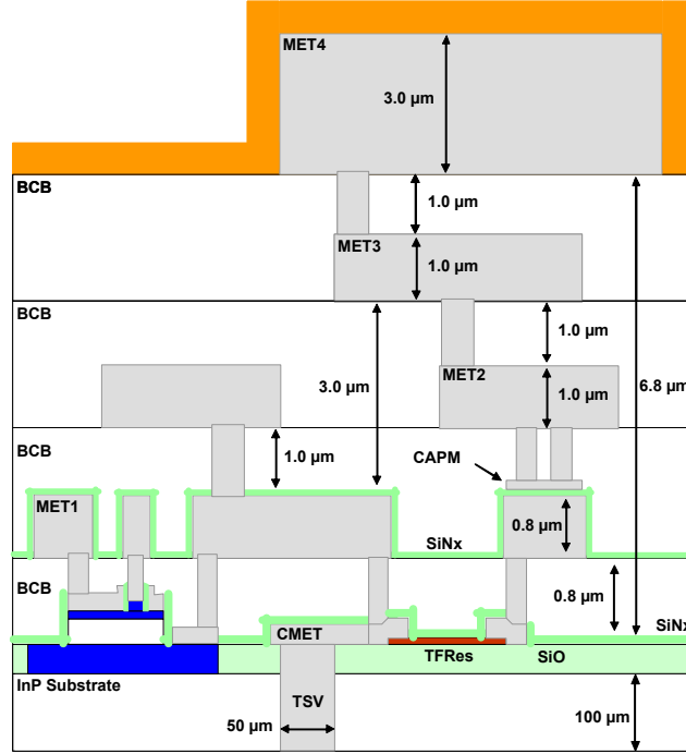
Figure 4.2: Cross-section of the 250 nm InP DHBT process by Teledyne.
