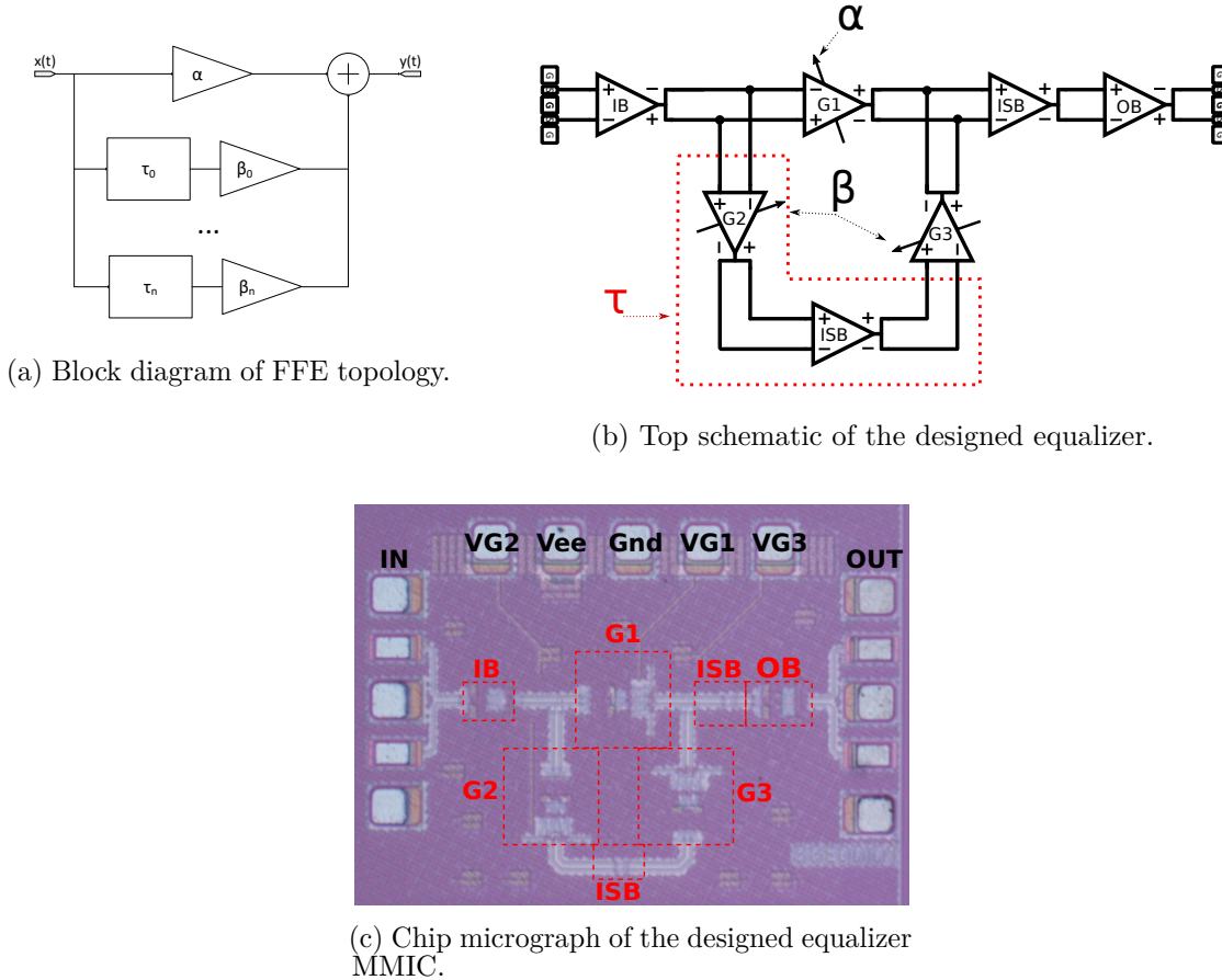
Figure 5.9: Implementation of the FFE Equalizer from block diagram to MMIC.
