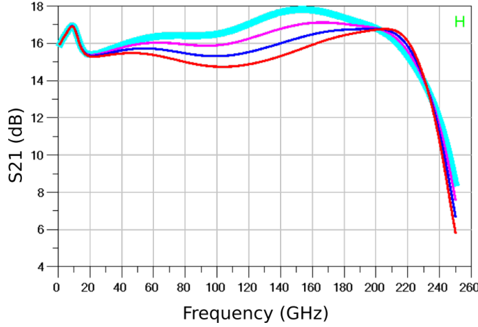
Figure 4.4: Effects of emitter inductance on gain of the DA. Cyan: 0 pH, purple: 2 pH, blue: 4 pH, red: 6 pH.
