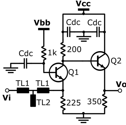
(a) Schematics of the CB TIA.
