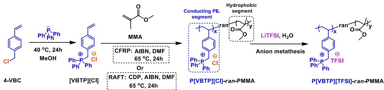
SCHEME 1 Synthetic scheme for synthesis of (A) P[VBTP][Cl]- ran -PMMA random copolymers via CFRP or RAFT polymerization and (B) P[VBTP][TFSI]- ran -PMMA copolymer by anion metathesis of the chloride to bis(trifluoromethane)sulfonamide (TFSI - ) ion [Color figure can be viewed at wileyonlinelibrary.com]
