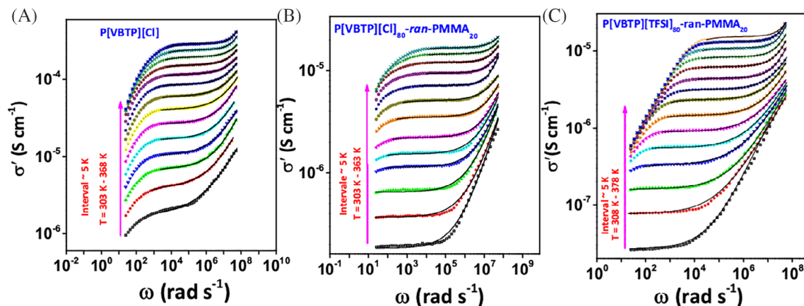
FIGURE 3 Real \sigma'(\omega) part of complex conductivity spectra of P[VBTP][Cl] (A), P[VBTP][Cl] 80-ran-PMMA 20 (B) and P[VBTP][TFSI] 80-ran-PMMA 20 (C) respectively in the frequency ranges from 4 Hz–8 MHz at different temperatures. The black lines in Figures 3(A)–(C) were fitted to Equation 1 [Color figure can be viewed at wileyonlinelibrary.com]
