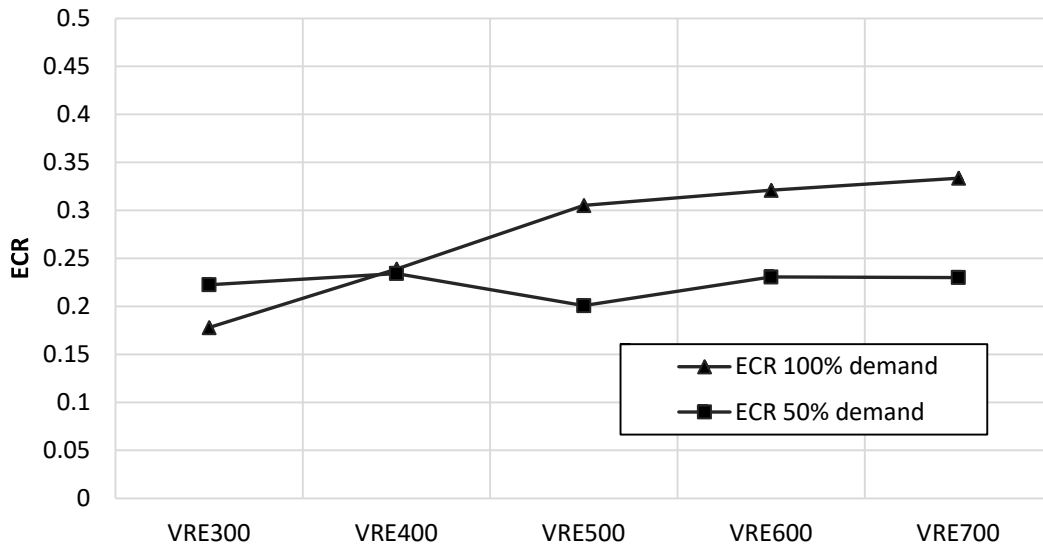
Fig. 17. Effective conversion ratio (ECR) for the DHHI in the MTDH systems with extraction plant
