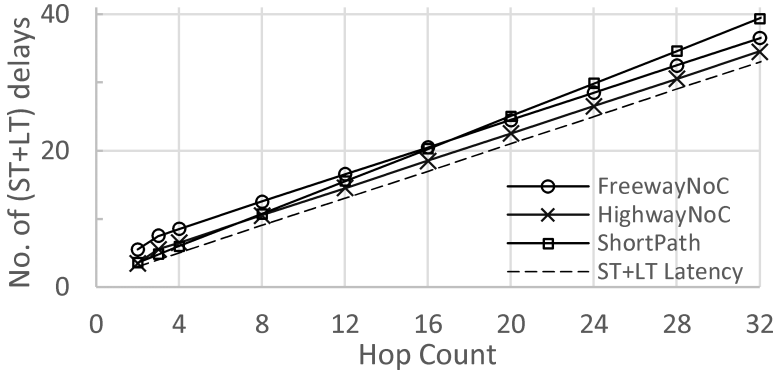
Figure 5.4: ZLL analysis with respect to hop count with the HighwayNoC, the FreewayNoC and the ShortPath networks versus an ideal network that has a delay of ST+LT per hop.
