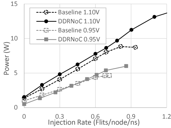
(a) Total power
