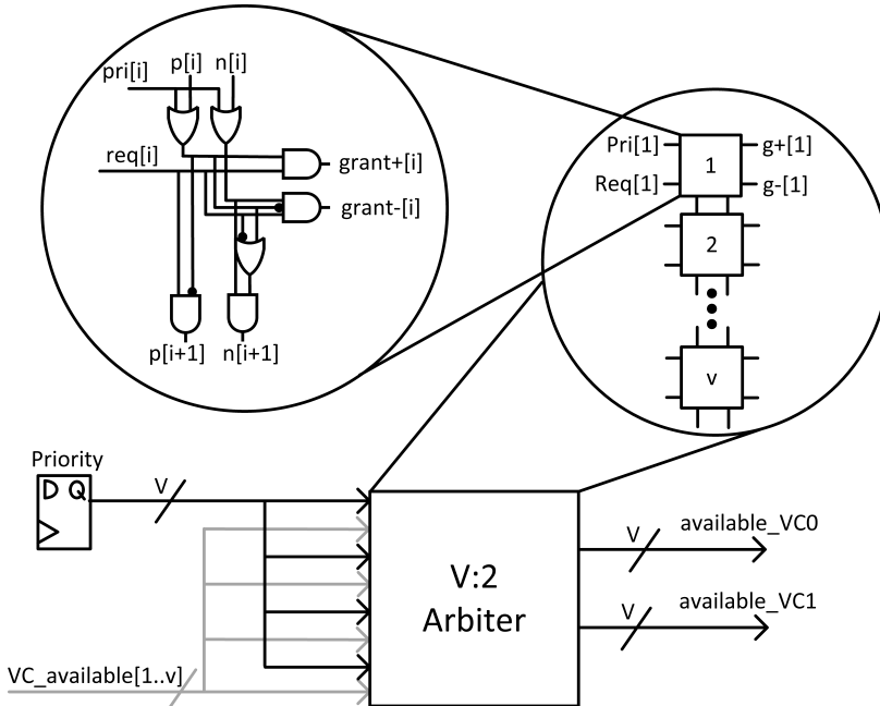
Figure 4.5: FreewayNoC VC selection
