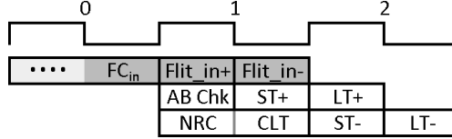
(b) Allocation Bypassing (AB) mode. Cycle-1, first half: NRC and checks for bypassing allocation. Cycle-1, second half: new FC is sent through the link and ST of first flit (+). Cycle-2: ST of the second flit (-) and LT of both flits.
