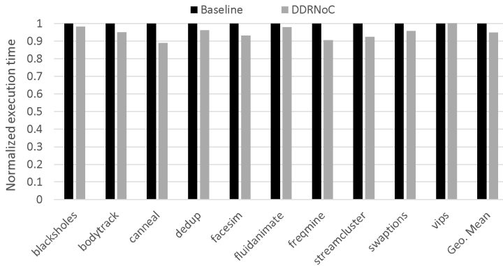
Figure 7.16: Normalized application execution time for PARSEC-2.1 benchmarks using full system simulations.
