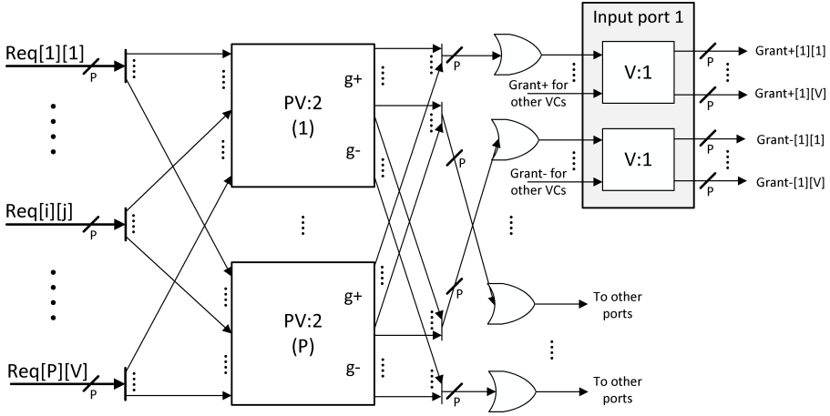
(a) DDRNoC dual grant Switch Allocator.
