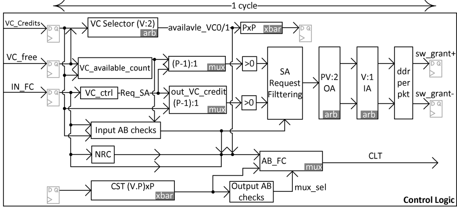
Figure 4.6: FreewayNoC control path analysis.
