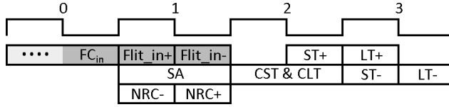
(a) Regular routing mode. Cycle-0: forwarded control (FC) signals arrive. Cycle-1: allocation and NRC performed, incoming flits buffered. Cycle-2: new FC signals go through ST (CST) and LT (CLT). Second half of Cycle-2 and Cycle-3: the two flits (+/-) perform ST and LT.
