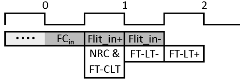
(c) FastTrack (FT) mode. Cycle-1, first half: FT checks, NRC and FC sent through the link. Cycle-1, second half: LT of first flit via FT path. Cycle-2, first half: LT of second flit via FT path.
