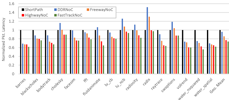
Figure 7.15: Normalized packet latency for application driven traffic.
