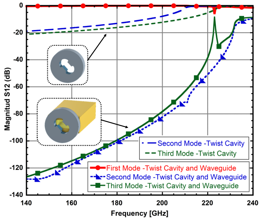
Figure 3.3. Propagation of the second and third mode for the standalone twist cavity, and the twist cavity connected to a rectangular waveguide. The third mode will introduce a resonance in the response.
