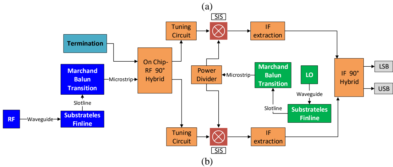
Figure 6.1. Future Outlook: Broadband mixer design. (a) Conceptual chip layout of waveguide to microstrip transition employing substrateless finlines developed in [Paper B] and the Marchand balun presented in Chapter 5. This transition could be used for RF and LO in a future SIS mixer design. (b) Conceptual block diagram for a sideband separating receiver employing the waveguide to microstrip transition shown in picture “a”. The complete chip may include 2 waveguides to microstrip transition for LO and RF, on chip RF hybrid, on chip power divider for the LO signal and tuning circuitry for the SIS.
