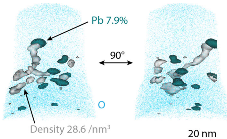
Fig. 10. Pb particles in the 600°C exposed material, visualized by 7.9 at.% Pb iso-concentration surfaces, and high-density volumes in connection with them, showed as 28.6 atoms/nm 3 iso-density surfaces (corresponding to 77.3 atoms/nm 3 when correcting for the detection efficiency of the LEAP). O atoms in blue show the extension of the analysis. The analysis is shown in two different directions. This is the same analysis that is shown in Figure 7.
