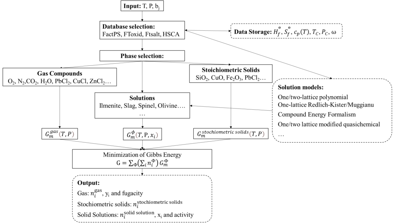
Figure 6. Schematic view of the calculation procedure in Equilib for multiphase multicomponent equilibrium calculations.
