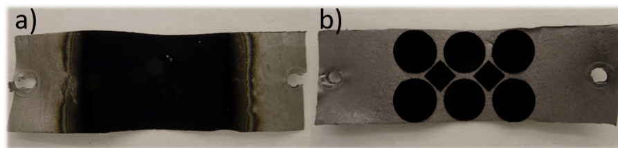
Figure 2.23: a) Unpatterned graphene CNT hybrid film and b) film with patterning.
