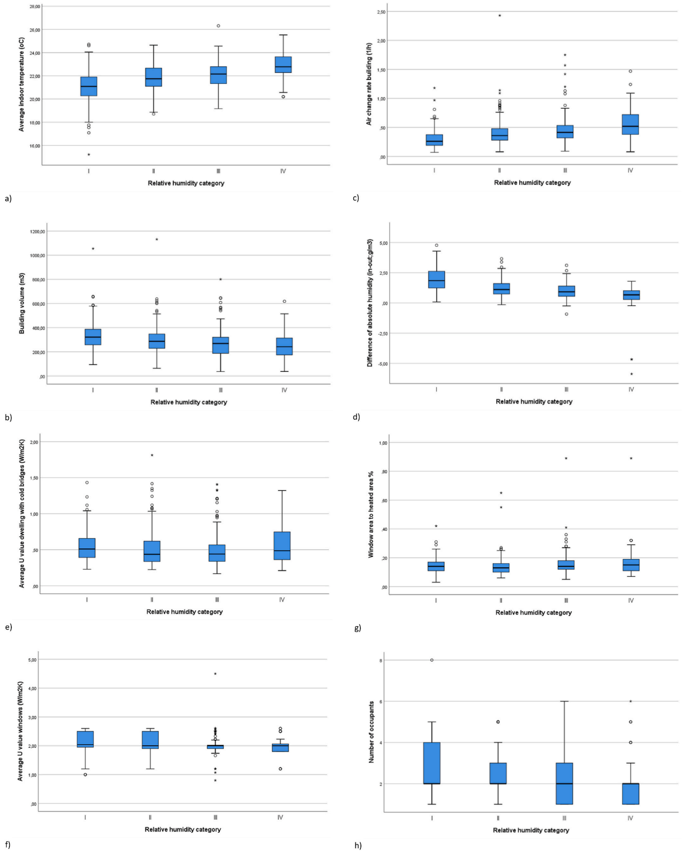
Fig. 3. Boxplots of different examined parameters: a) average indoor air temperature (°C), b) the total heated building volume (m 3 ), c) the building level ventilation air change rate (h -1 ), d) the average difference between indoor and outdoor absolute humidity (indoor moisture supply; g/m 3 ), e) the average U-value of the dwelling (thermal bridges; W/m 2 K), f) the average U-value of the windows (W/m 2 K) g) the window area to heated area ratio and h) the number of occupants, for the four RH assessment categories. Category I: >30%, Category II: >25%, Category III: >20%, Category IV: >0%.
