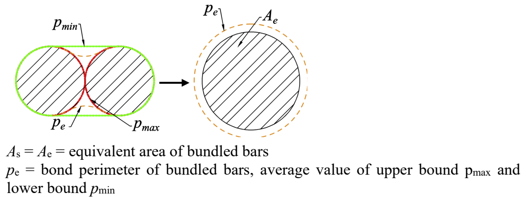
Figure E.6 Scheme of the minimum, maximum and average perimeters and the equivalent area and perimeter for the bundled reinforcement bars.
