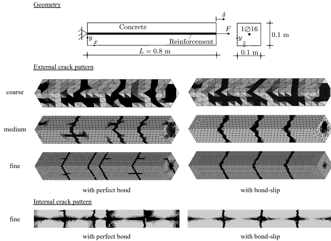
Figure 3.10 External and internal crack pattern in reinforced concrete prism subjected to a tensile load; effect of mesh density when assuming perfect bond or a bond-slip relation. Based on Grassl et al. (2018).
