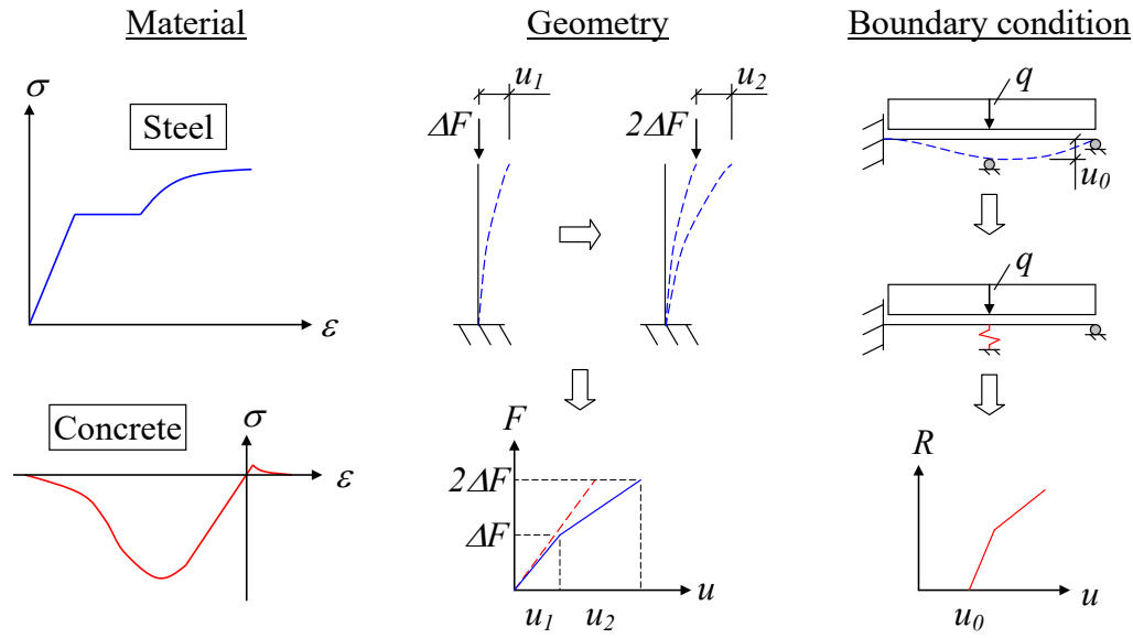
Figure 3.1 Examples of possible types of non-linearity in a FE analysis.
