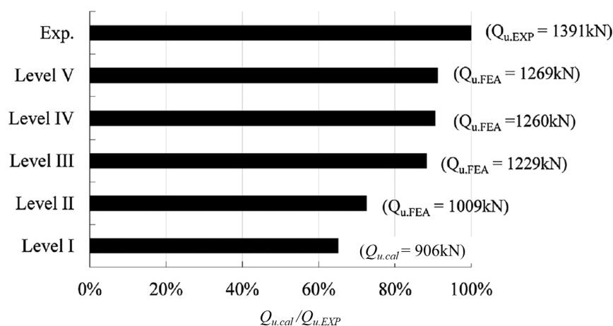
Figure 7.24 Load-carrying capacity, limited by punching shear, of the cantilever RC slab DR1-a with assessment at different levels, compared with experimental results. From Plos et al. (2017).
