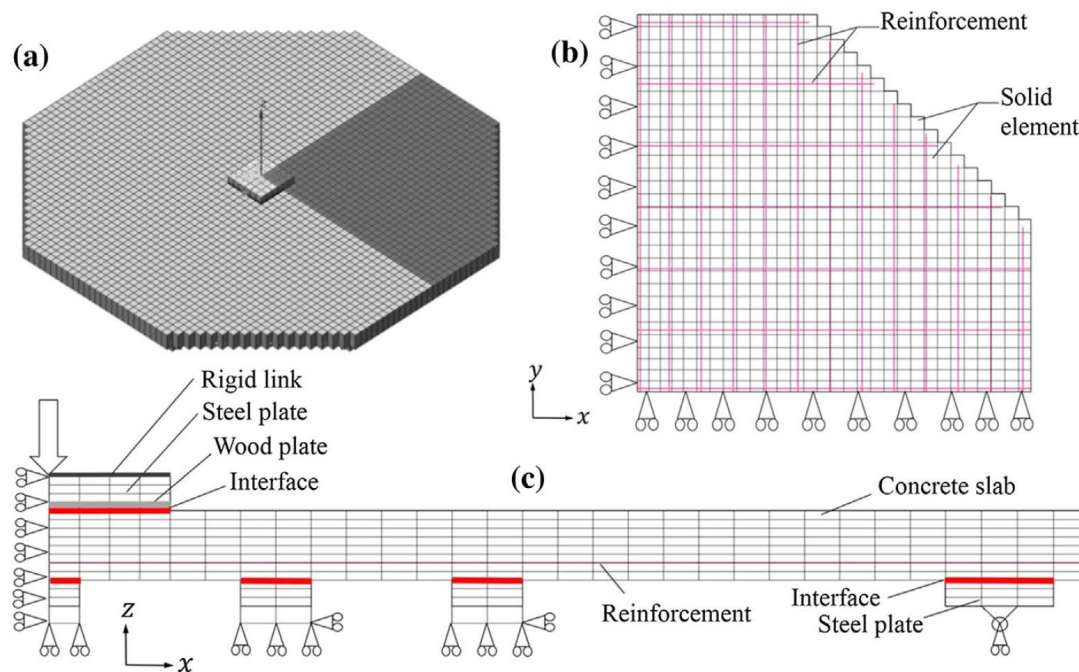
Figure 7.7 Non-linear continuum element model of the two-way slabs for level IV and V; (a) isometric view with the modelled quarter of the slab marked; (b) top view; (c) side view. From Plos et al. (2017).
