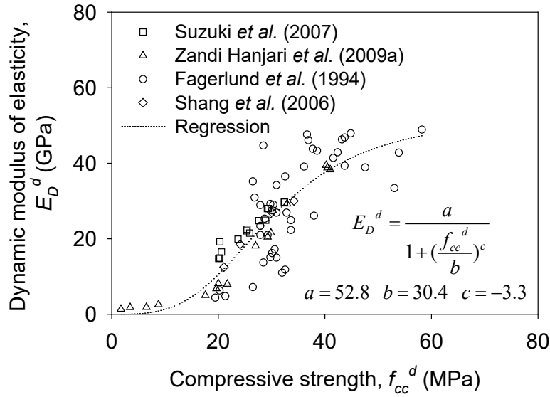
Figure B.1 Correlation between compressive strength and dynamic modulus of elasticity for frost-damaged concrete.
