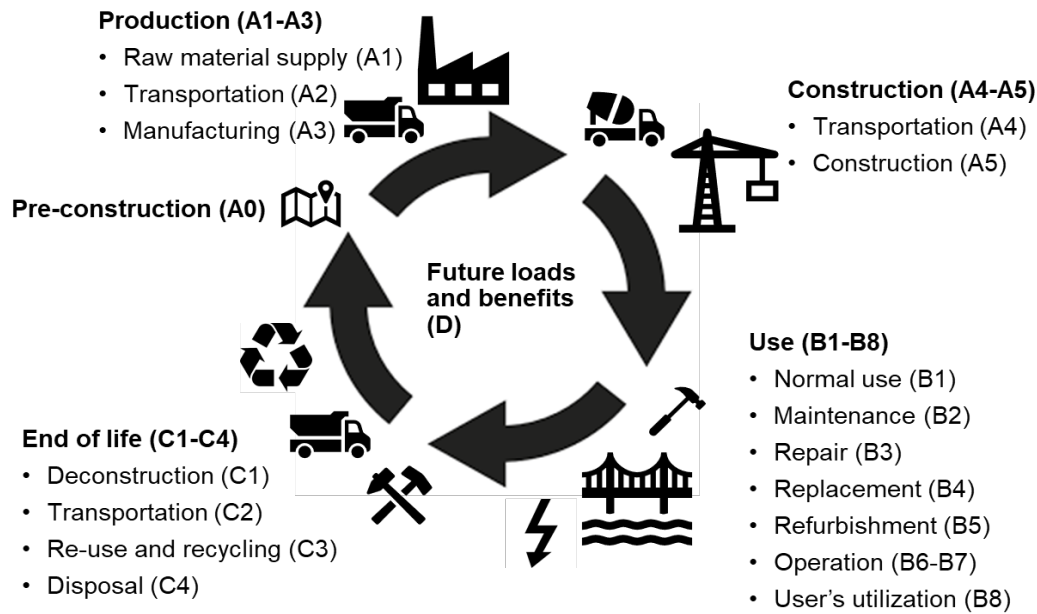
Figure 2.2. Schematic overview of the life cycle stages of a civil engineering works project and their classification in modules according to EN 15643-5:2017 [45], reproduced from Paper B [2].
