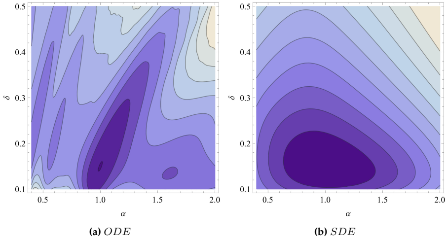
Figure 3.1: Illustration of the regularization using SDEs in the Lotka-Volterra predator-prey model. The two plots show the level curves of the likelihood function in the parameter estimation problem using the ODE setting (a) and the SDE setting (b). In (a) there are several local minima to where a local optimization algorithm might converge.
