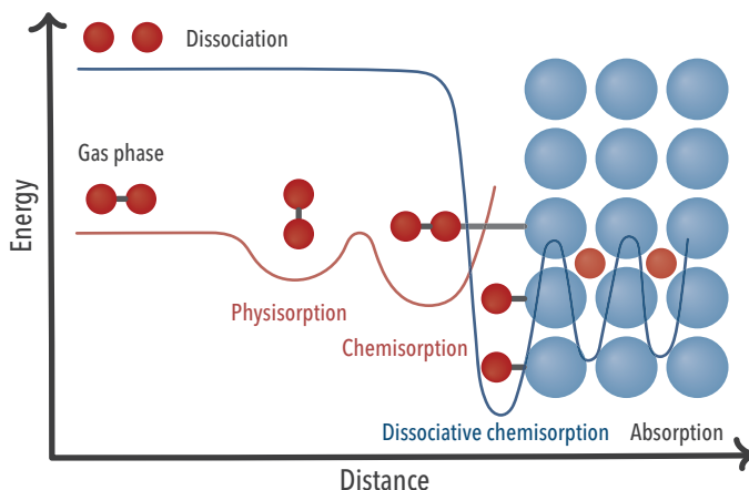
Figure 3.1: Surface adsorption. The energy landscape of molecular surface adsorption is dictated by the van der Waals attraction and Pauli repulsion (red line), and the dissociation barrier (blue line). Surface adsorption occurs either through molecular physisorption without breaking molecular bonds or through associative or dissociative chemisorption, which entails the formation of covalent bonds with surface atoms. Dissociated species may also diffuse into the lattice, where a diffusion jump is associated with a specific energy barrier. Figure adopted from reference 59 .
