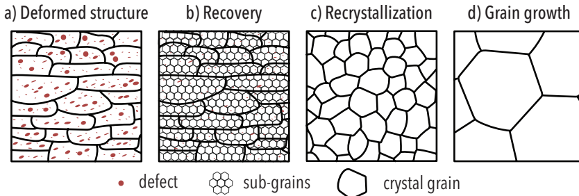
Figure 2.4: The steps of morphological transitions of deformed polycrystals subject to thermal treatment include; a) a structure with deformed grains formed by cold working (red dots are illustrating defects), b) recovery through decreasing defect density and sub-grain nucleation (drawn as a honeycomb lattice), c) recrystallization of the grain morphology and d) competitive grain growth. Figure is adapted from reference 46 .
