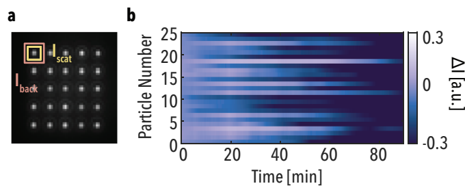
Figure 7.4: Plasmonic nanoimaging. a) 5 x 5 particle array of 150 nm diameter Cu nanoparticles, where the pixel boxes for intensity integration ( I_{scat} and I_{back} ) are indicated. b) Time evolution of the integrated scattering intensity change, \Delta I , of the 25 Cu nanoparticles during 90 minutes oxidation in 1 % O_2 at 150 °C.
