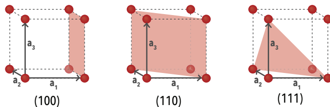
Figure 2.2: The three simplest cubic lattice planes: (100), (110) and (111). Examples of three lattice planes (pink surfaces) in a simple cubic unit cell and their Miller Indices: (100), (110) and (111), respectively.
