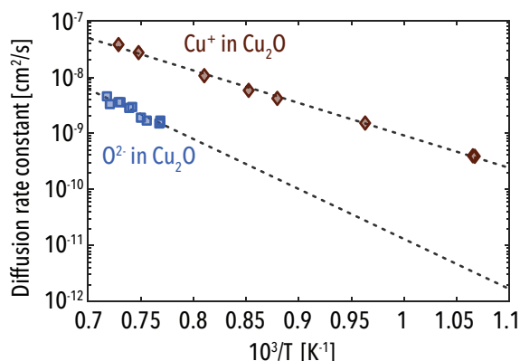
Figure 3.6: Diffusion rate constants of oxygen and copper ions in Cu 2 O. The diffusion rate constant for copper (Cu + , red diamonds) and oxygen ions (O 2- , blue squares) in Cu 2 O
