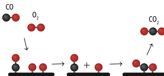
Figure 4.2: CO oxidation elementary reaction steps. The CO oxidation reaction on a catalyst follows the steps; dissociative surface adsorption of O_2 and associative adsorption of CO, oxidation of the CO molecule into CO_2 , and desorption of the newly formed CO_2 molecule. Figure adopted from reference 35 .
