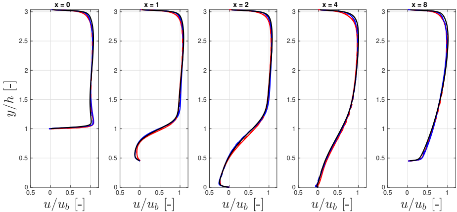
Figure 3.2: Hybrid RANS/LES of Periodic Hills at Re_h = 10595 . Effects of turbulence model and numerical properties on streamwise velocity u . HYB0 Ref scheme (—), HYB0 LD2 scheme (- - -), SA-DDES Ref scheme (—), SA-DDES LD2 scheme (- - -), Reference LES [60](—).
