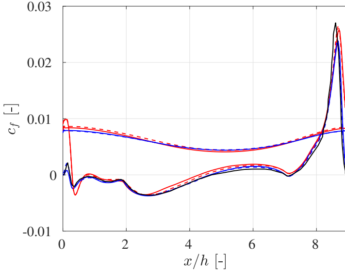
Figure 3.4: Hybrid RANS/LES of Periodic Hills at Re_h = 10595 . Effects of turbulence model and numerical properties on skin friction coefficient. HYB0 Ref scheme (—), HYB0 LD2 scheme (- - -), SA-DDES Ref scheme (—), SA-DDES LD2 scheme (- - -), Reference LES [60] (—).
