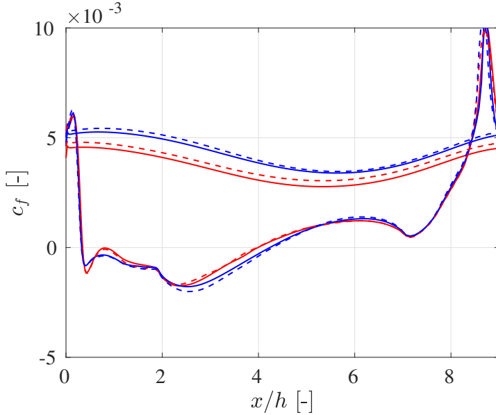
Figure 3.7: Hybrid RANS/LES of Periodic Hills at Re_h = 37000 . Effects of varying turbulence model and numerical properties on skin friction coefficient. HYB0 Ref scheme (—), HYB0 LD2 scheme (---), SA-DDES Ref scheme (—), SA-DDES LD2 scheme (---).
