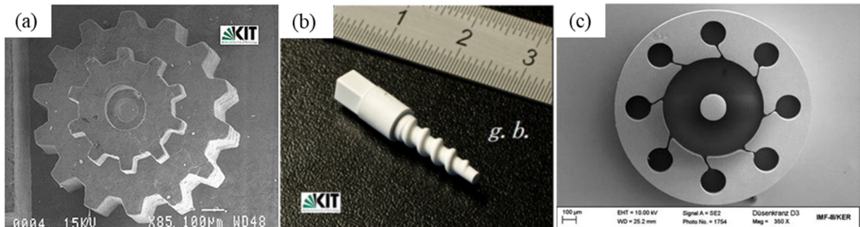
Fig. 8. a: a ceramic micro gear wheel injection-moulded using LIGA mould inserts (Reprinted with permission from [81]); b: a dispenser screw made of \text{ZrO}_2 (Reprinted with permission from [81]); and c: SEM image of a nozzle plate made of sintered \text{ZrO}_2 (Reprinted with permission from [82]).
