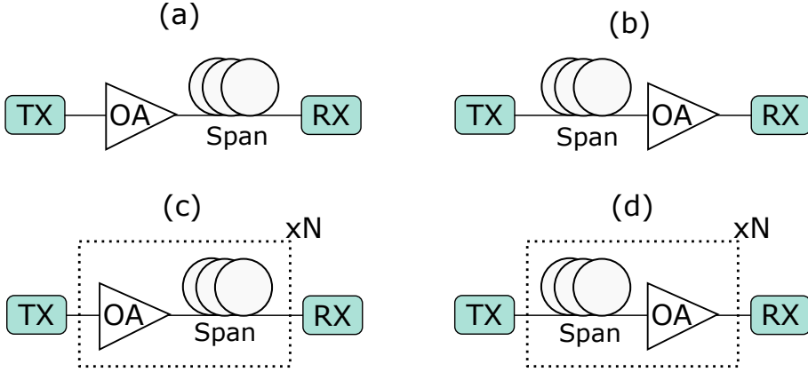
Figure 3.1: Different configurations in which optical amplifiers (OA) can be used in a fiber-optic communication link, a) booster amplifier, b) pre-amplifier, c) inline - type A amplifier, d) inline - type B amplifier. TX - transmitter and Rx- receiver.
