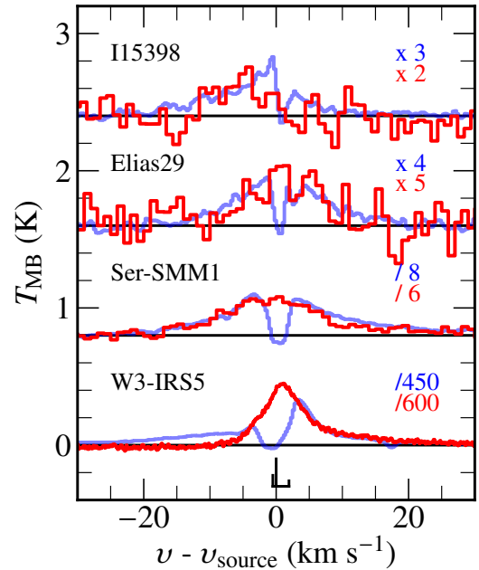
Fig. 15. Comparison of HIFI spectra of the H 2 O 1_{10}-1_{01} 557 GHz line (blue) and the OH 1834 GHz triplet (red) toward a number of low and high-mass regions. The splitting of the three OH lines in the triplet and their relative strength are indicated at the bottom of the figure. Data from Kristensen & Wampfler (priv. comm.).
