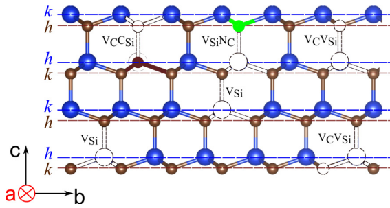
FIG. 1. Schematic representation of defect configurations in 4H-SiC. Blue, brown, and green spheres denote silicon, carbon, and nitrogen atoms, respectively. Vacancy sites are shown as hollow spheres. The planes labeled h and k indicate the symmetry of lattice sites.
