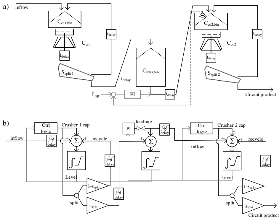
Figure 5.6: a) Flowsheet of the originally modeled plant, and b) the flowsheet implemented for the simulation of the plant
