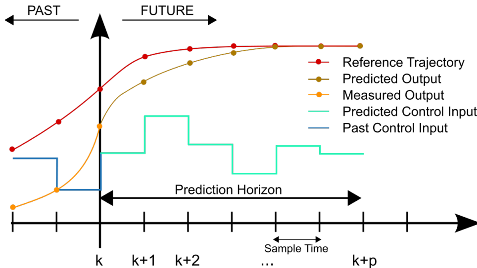
Figure 4.6: A graphical representation of MPC by M. Behrendt. licensed under CC 3.0
