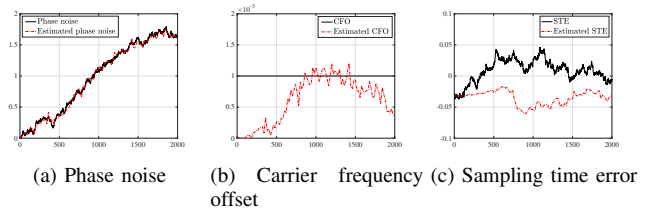
Fig. 2. Estimation of PN, CFO and STE parameters for a block of 2000 symbols, after running Phase I of the proposed algorithm based on pilot symbols.
