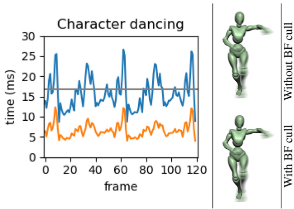
Fig. 10. Performance comparison of using back-face culling on the character dancing scene with a 1024×1024 resolution and opaque textures. The blue graph shows the time per frame without back-face culling and the orange graph shows the time per frame with back-face culling. As expected, the average time per frame is significantly shorter with back-face culling at 6.67 ms compared to 15.72 ms without. The grey horizontal line indicates 60 FPS. (For interpretation of the references to color in this figure legend, the reader is referred to the web version of this article.)
