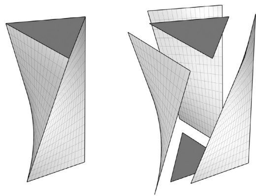
Fig. 3. Left. A triangular prism shape represents the trajectory of a moving triangle. Right. The prism has been cut open to reveal the two triangles and three bilinear patches it is composed of in our representation. The dark grey triangles represent the start and end positions of the triangle's motion.
