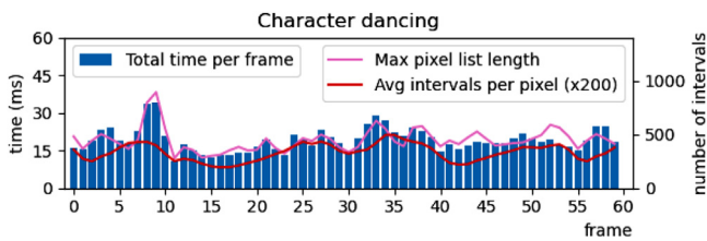
Fig. 15. Time per frame of the first 60 frames of the character dancing scene related with interval counts per frame. The time per frame is largely dependent on the number of intervals per frame and on the length of the longest pixel lists. The average number of intervals considers also empty pixels hence the magnification \times 200 .
