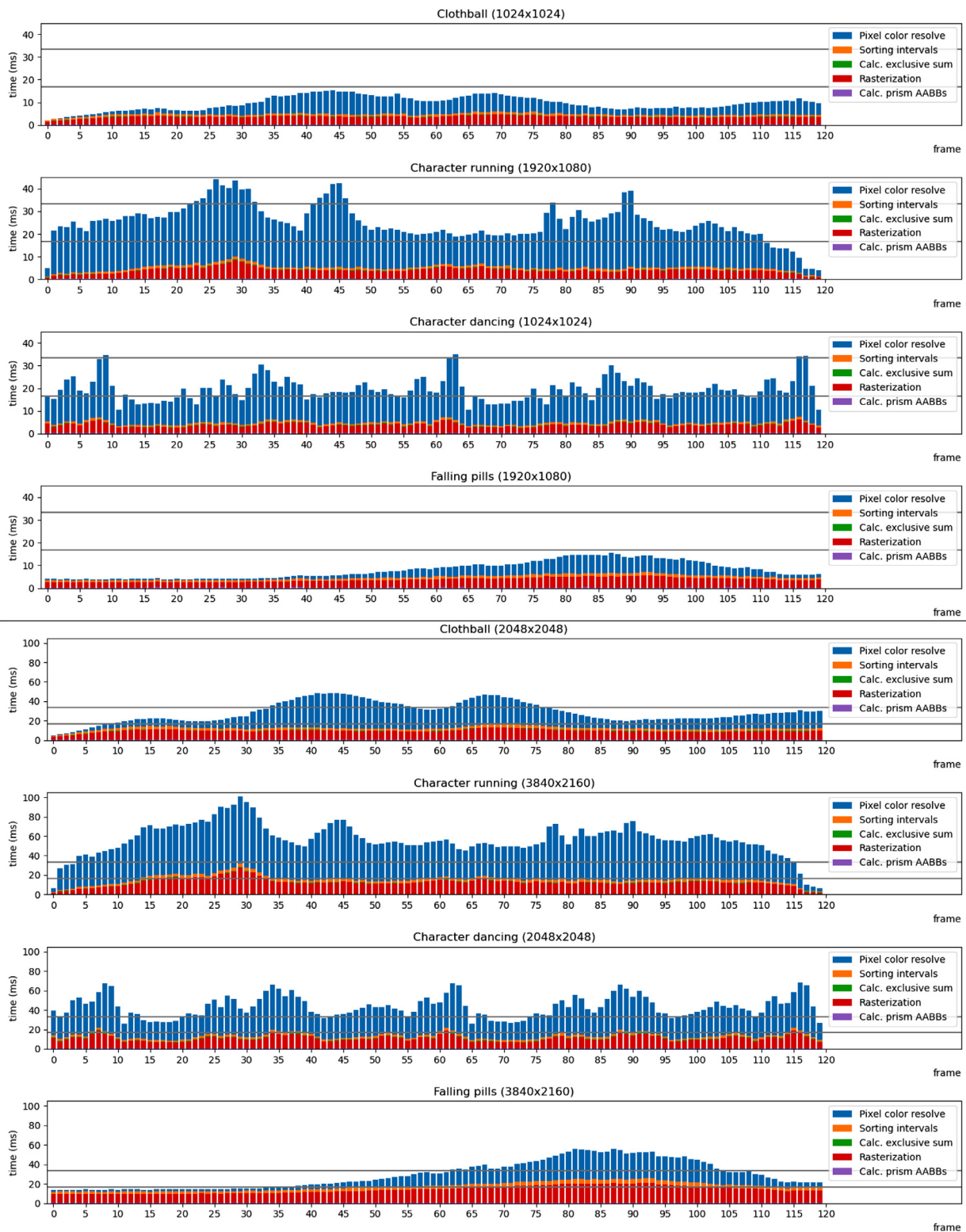
Fig. 13. (Top) Per frame timings for tested scenes. For screen resolutions of 1920 \times 1080 and 1024 \times 1024 (top), the timings generally stay within 30 frames per second and within 60 frames per second for some scenes. For resolutions of 3840 \times 2160 and 2048 \times 2048 (bottom), timings go up to 100 ms in the character running scene. The grey horizontal lines indicate 60 and 30 FPS respectively.
