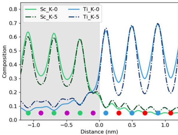
Fig. 6. The effect of beam spreading on the observed sharpness of the interfaces. Here, the data from the 100 nm sample is replotted from Figure 5 to show only the Sc-K to Ti-K lines at tilts of 0° and 5°. The colored dots present the atomic column locations of every element, and the gray-shaded region shows the location of the DSO layer.
