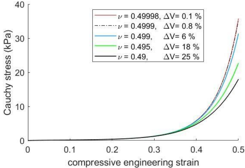
Figure 18. The effect of Poisson's ratio; tissue stiffness and volume change for Ogden model with VFLAG=0 in the material keycard. The delta value corresponds to the volume change.
