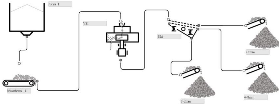
Figure 9. A crusher plant overview map of the Källareds VSI subsection made in the Rocksim Plantsmith process simulator.
