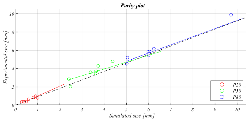
Figure 20 A parity plot of the P20, P50 and P80 values from the experimental data compared to the simulated data using the developed models. (Paper C)
