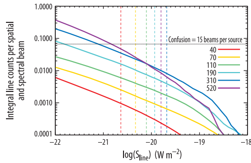
Fig. 7 Integral spectral line counts per spatial beam and spectral resolution element (at R = 300 ) for each Origins /OSS band (wavelengths in \mu\text{m} ; see legend). The detection limit of the deep survey in each band is shown by the vertical dashed lines. The nominal confusion limit for imaging, 15 beams per source, is shown as the dotted horizontal line. In all bands, the counts for the deep survey are well below the confusion limit.
