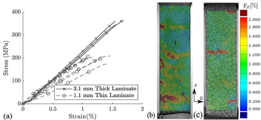
Figure 7. (a) Tensile stress-strain curves of the thick and thin CF-PP TBDCs, (b) DIC strain field of thin specimen which shows larger distribution of hotspots and (c) DIC strain field of a thick specimen with low number of hot spots.
