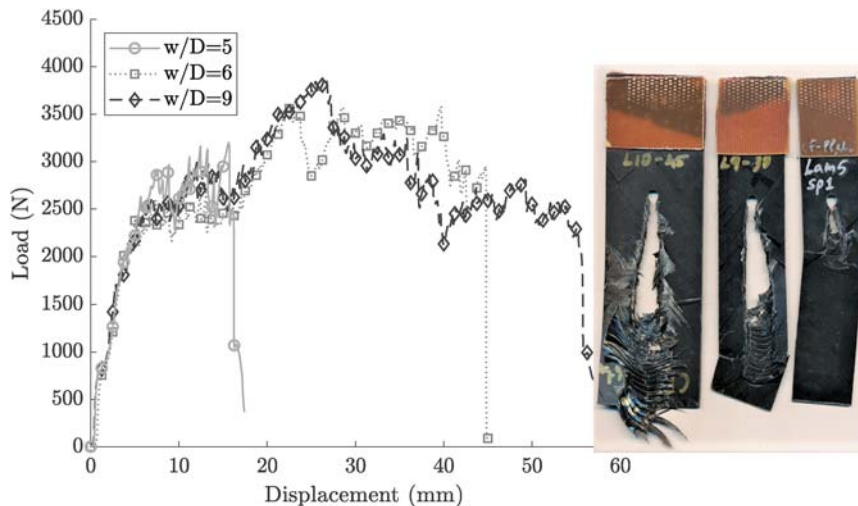
Figure 14. (left) Force vs displacement curves for different w/D ratios, (right) extent of Tearing damage in the specimen with different w/D ratios.
