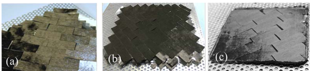
Figure 2. Manufacturing process of TBDCs, (a) single UD CF-tape discontinuous layer, (b) QI stack of discontinuous composite and (c) consolidated TBDC laminate.
