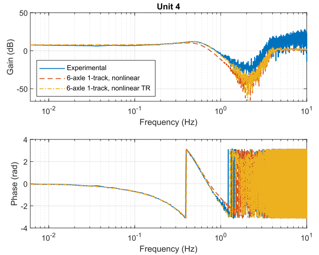
FIGURE 15. The input-output gain and phase difference of the single-track 6-axle vehicle model with/without modeling the tire relaxation (TR). The input is the road wheel steering angle, and the output is the yaw rate of unit 4. Consideration of the tire relaxation improved the yaw rate response.
