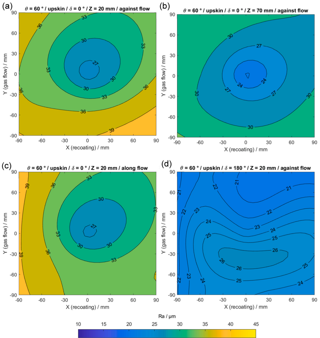
Fig. 12. Conotur plots of surface roughness (Ra) variation predicted by neural network model across the build for 60° upskin surfaces of LPBF Ti-6Al-4V alloy products built in EOS M280 machine.
