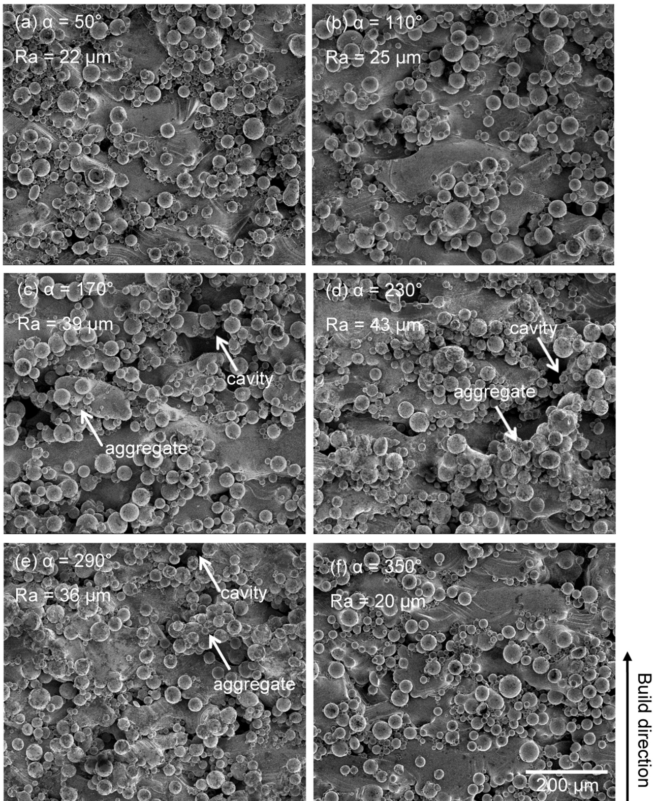
Fig. 9. SEM images of selected facets in specimen L-3-B on 60^\circ upskin surfaces (located at left column, third row and bottom layer of the stacks). Corresponding surface profiles and surface texture parameters are presented in Fig. 10.
