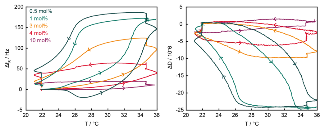
Figure 4. QCMD plot (left: resonance frequency, right: dissipation) of PNIPAM- co -MBAM with 0.5 mol % (dark green), 1 mol % (green), 3 mol % (orange), 4 mol % (red), and 10 mol % (purple) crosslinker content.
