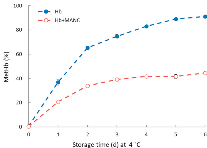
Fig. 4. Auto-oxidation of herring Hb during incubation with Duralox MANC. Hb was diluted to 5 \mu\text{M} in 50 mM phosphate buffer, pH 6.3 and incubated at 4 °C. The final concentration of Duralox MANC was 0.5 g/L.
