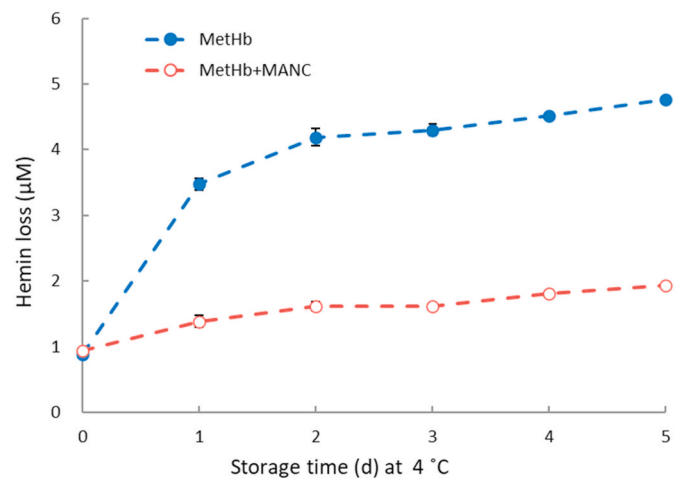
Fig. 5. Spontaneous hemin loss from herring metHb. MetHb was diluted to 5 \mu\text{M} in 50 mM phosphate buffer, pH 6.3 and incubated at 4 °C. The final concentration of Duralox MANC was 0.5 g/L.
