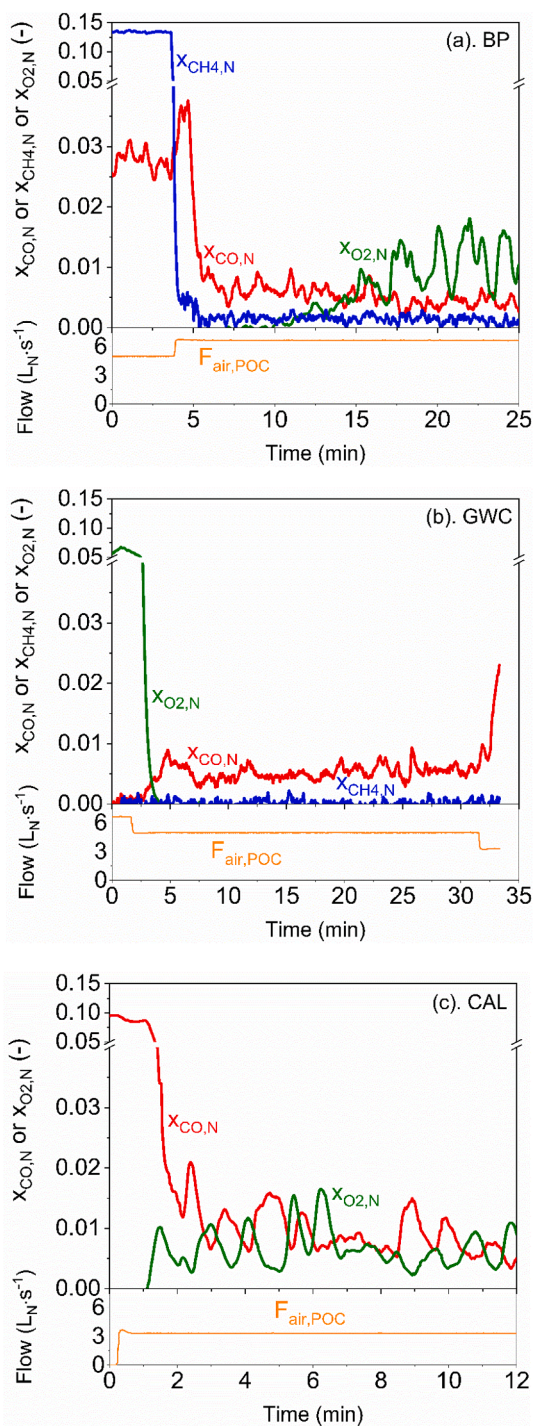
Fig. 10. Tests showing simultaneous low concentrations of O 2 , CO and/or CH 4 at the outlet of POC using (a) 67 kW th BP pellets with SC ore, (b) 80 kW th GWC wood char with SC ore and (c) 65 kW th CAL coal with Sinaus ore; CH 4 concentration was not measured for CAL and H 2 was not measured for all the three fuels for these results.
