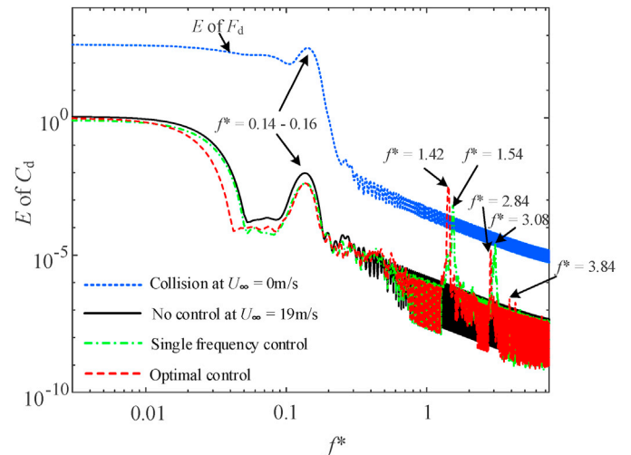
Fig. 10. Power spectra of drag force under different control parameters. Single frequency control: f^* = 1.54, U_{afc}^* = 0.67 ; Optimal control: f_1^* = 1.42, f_2^* = 3.84, U_{afc1}^* = 0.67, U_{afc2}^* = 0.63 .
