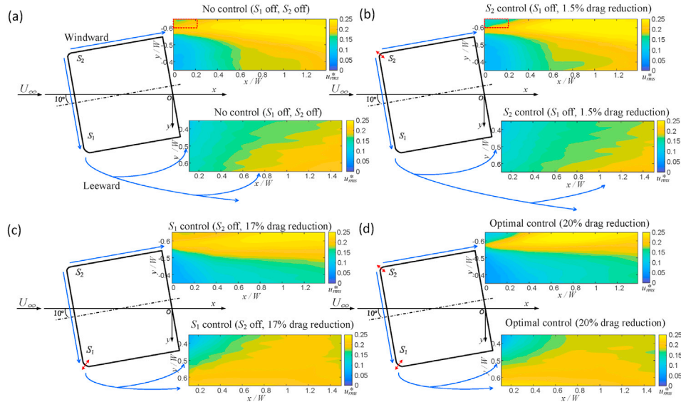
Fig. 12. Iso-contours of u_{rms} in the wake of bluff body. Refer to Fig. 11 for the control parameters in (a), (b), (c) and (d). The contour resolution is \Delta = 0.01 . The red arrows indicate the actuation position and the blue lines represent the flow separation around bluff body. U_\infty = 19 m/s. (For interpretation of the references to color in this figure legend, the reader is referred to the Web version of this article.)
