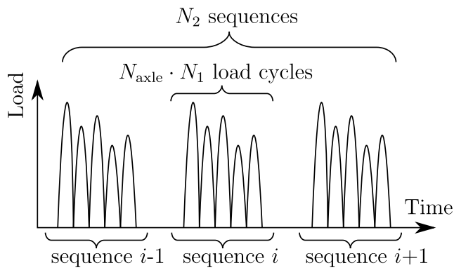
Fig. 7. Illustration of load collective generation based on N_2 identical load sequences, where each load sequence includes N_{axle} \cdot N_1 different load cycles.
