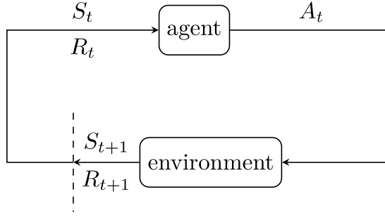
Figure 5.1: An illustration of the interaction between the agent and the environment in the MDP framework.
