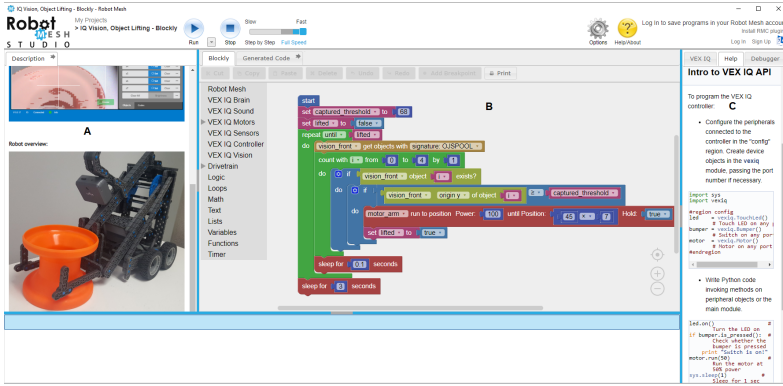
Figure 2.1: Screenshot of the Robot Mesh Studio IDE [67] with three panes. Pane A provides a rich-text description of the mission, Pane B shows the actual mission expressed in a DSL with Blockly syntax, and Pane C shows help text or alternatively the debugger or an overview on the current robot configuration.
