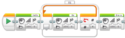
Figure 2.3: Specifying a loop in LEGO Mindstorms EV3.
