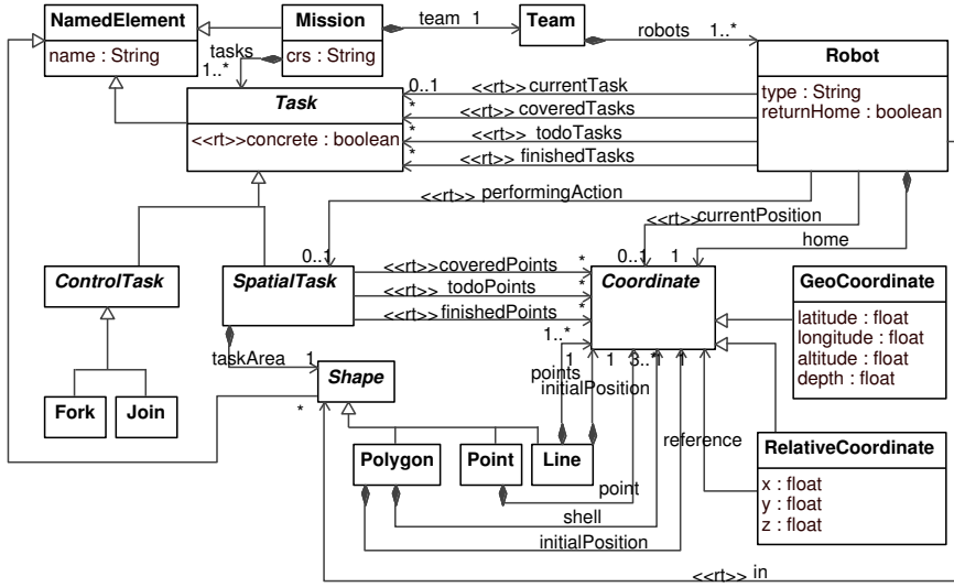
Figure 4.4: The annotated class diagram of the MML mission layer (context layer remains unchanged and is not shown).
