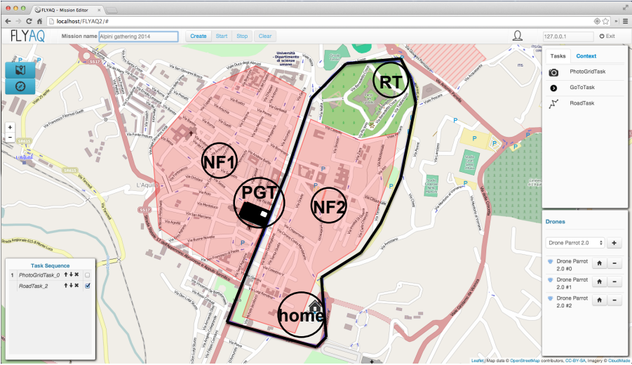
Figure 3.6: A patrolling mission in FLYAQ, where a drone follows a street, repeatedly takes photos (at specified distances), and avoids no-fly zones. NF1 and NF2 are no-fly zones, RT is road task to follow a street while PGT is photo grid task indicating where photos can be taken. (from [11])
