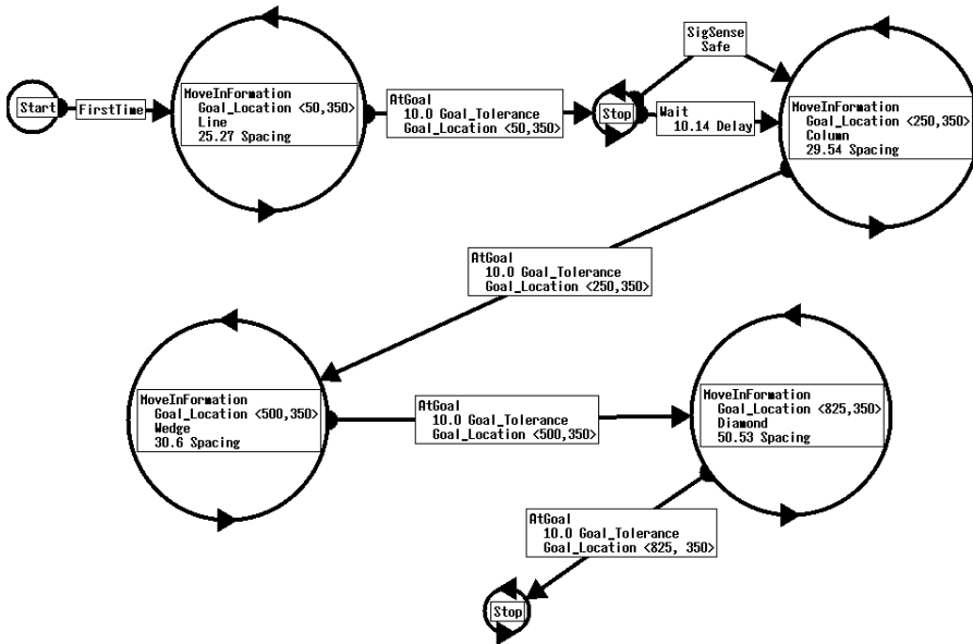
Figure 3.4: Graph-based state transition diagram for a multi-robot scouting mission in MissionLab (from [158])
