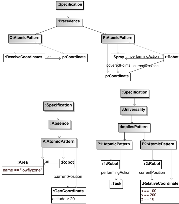
Figure 4.8: Three examples of temporal specifications as instances of MSL.
