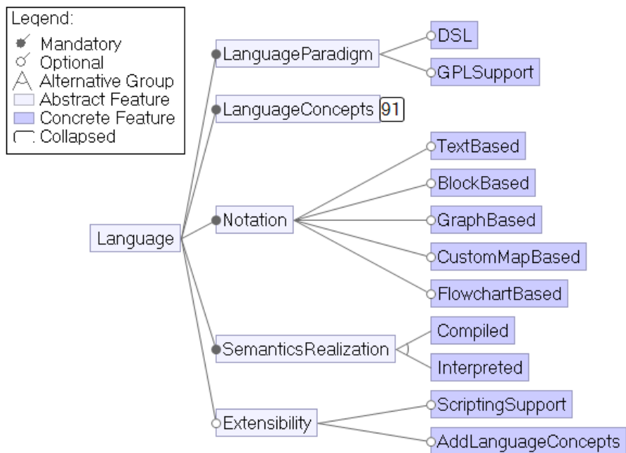
Figure 3.9: General language characteristics identified
