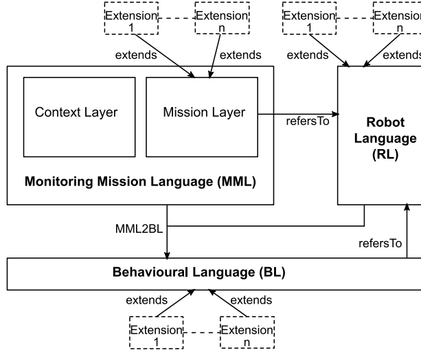
Figure 4.1: The family of FLYAQ DSMLs (adapted from [35]).
