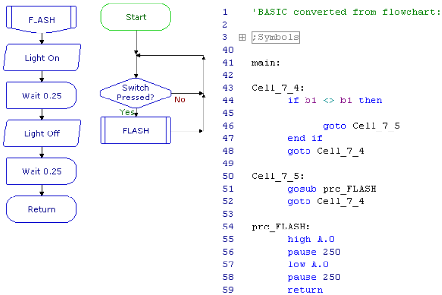
Figure 3.3: Left: A mission specified in PICAXE's flowchart-based language. Right: generated target code in PICAXE's BASIC language (from [70])
