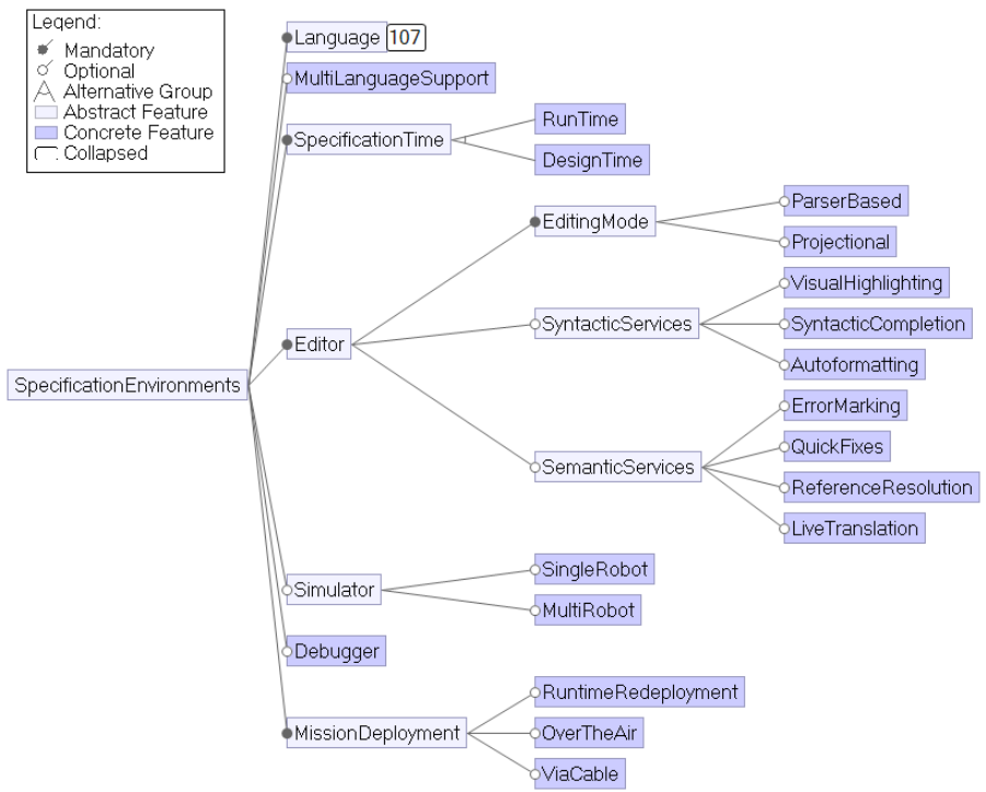
Figure 3.7: Overview of the features (133 features in total)
