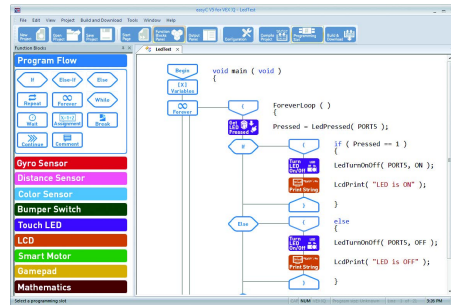
Figure 3.8: Visual and textual syntax side-by-side in EasyC's projectional editor (from [128]).
