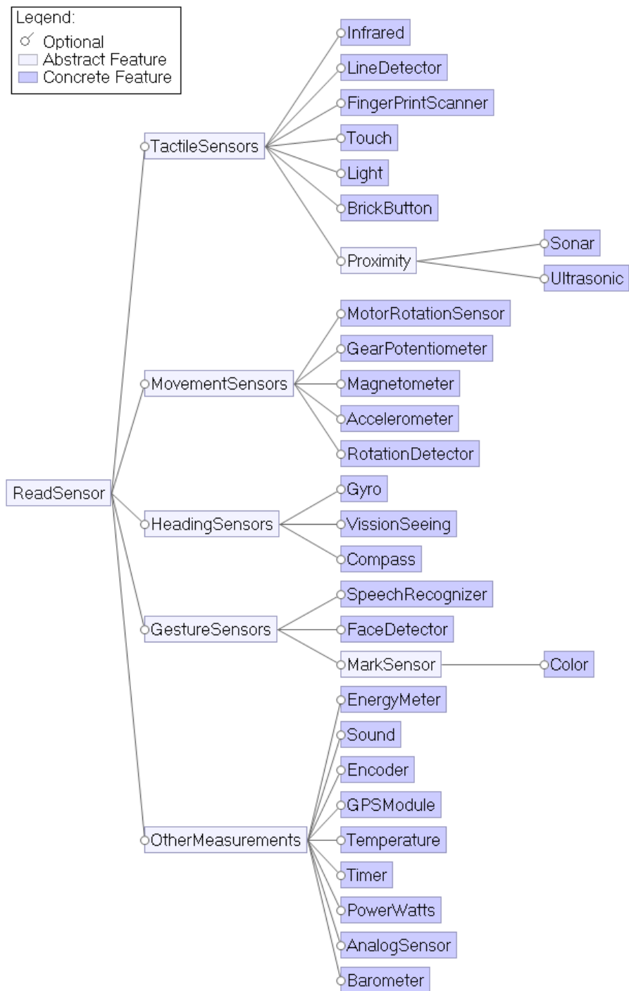
Figure 3.14: Sensors with language constructs for reading data
