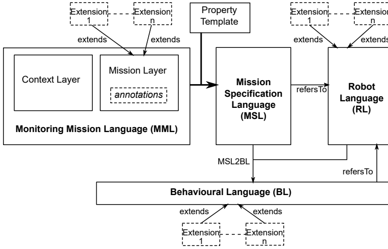
Figure 4.3: Overview of the approach as an extension of the FLYAQ platform.
