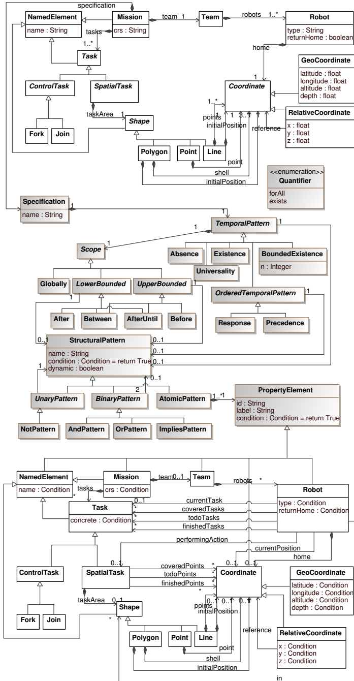
Figure 4.5: The generated metamodel of MSL without extensions.
