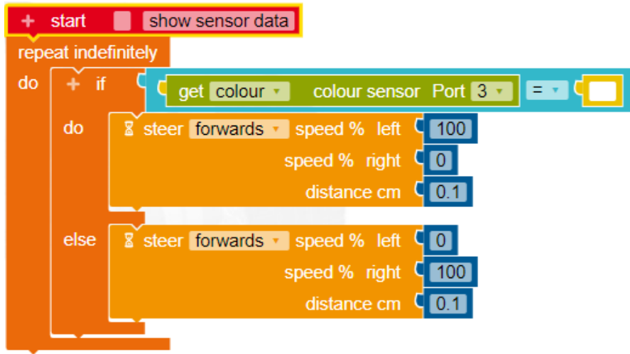
Figure 3.1: Block-based mission of a robot patrolling a perimeter wall, expressed in Open Roberta
