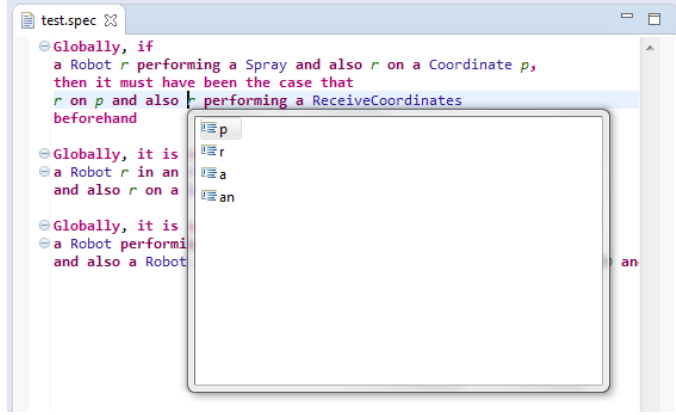
Figure 4.6: Screenshot of the MSL in Xtext.
