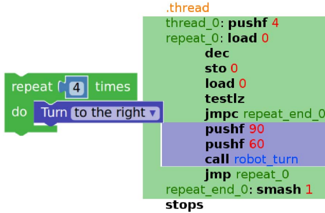
Figure A.2: Example of Metabot’s visual notation (left), together with generated assembler code (right) from [137]
