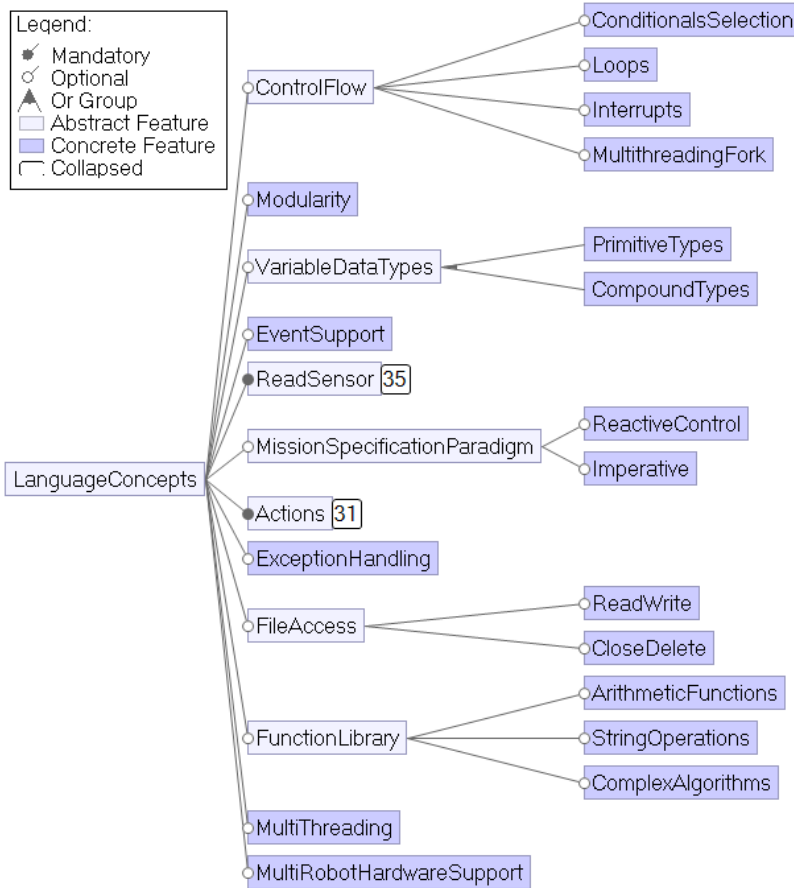
Figure 3.10: Language Concepts
