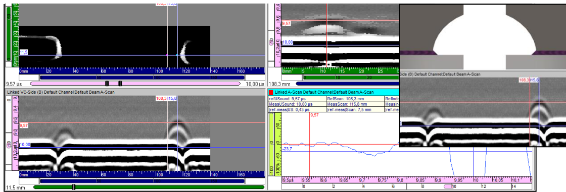
Scanning and visualisation software – two cracks appear in the image, with the shape of an arc. Back wall echo is looking like horizontal black and white stripes. The positions where the backwall pattern tend to bend downwards in the bottom left pane, are beginning and the end of the fillet welds.
