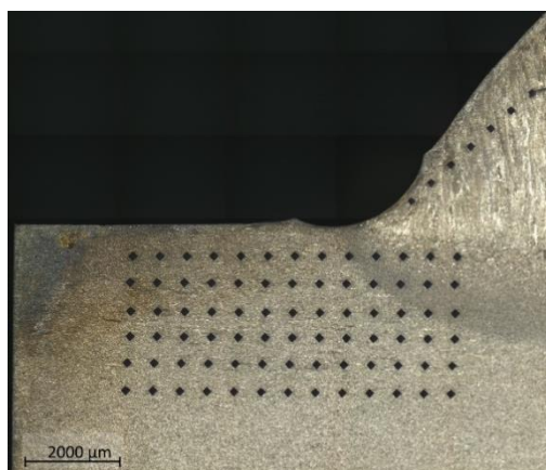
Figure 14: Micro-hardness tests and results.
