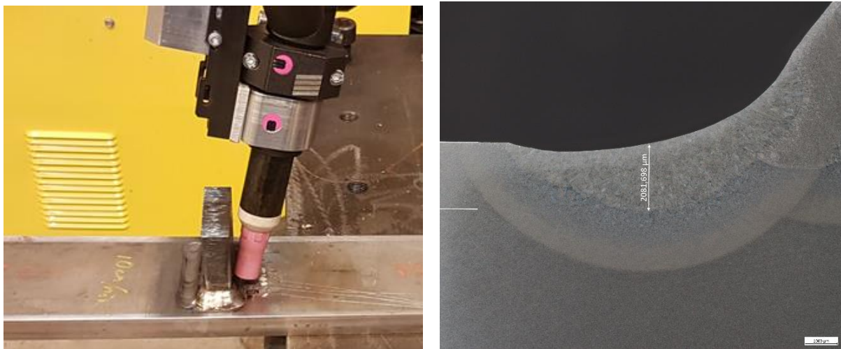
Figure 4. Left: TIG-torch direction for fatigue crack repair. Right: TIG-reweld transition region.
