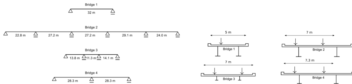
Figure 8. The four case-study bridges.
