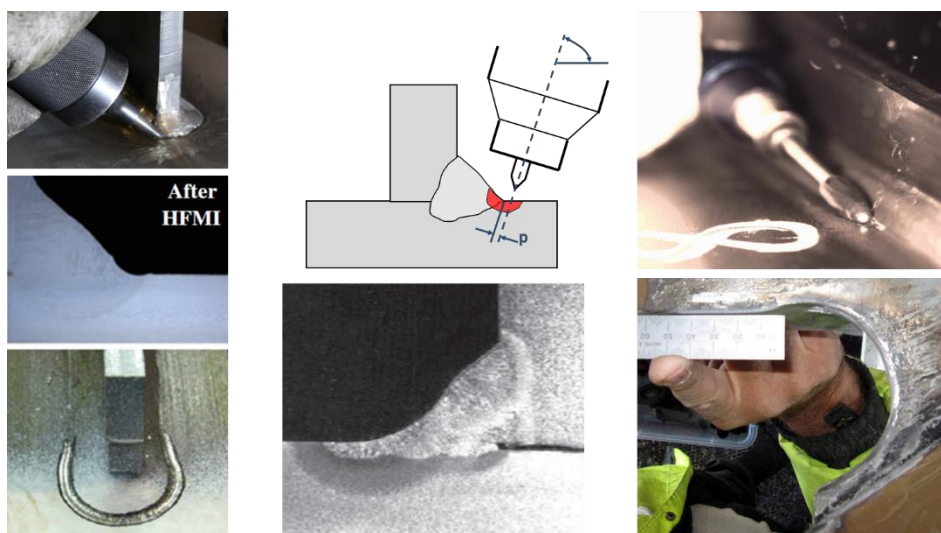
Figure 7. Methods for fatigue life extension used in the LifeExt project.
