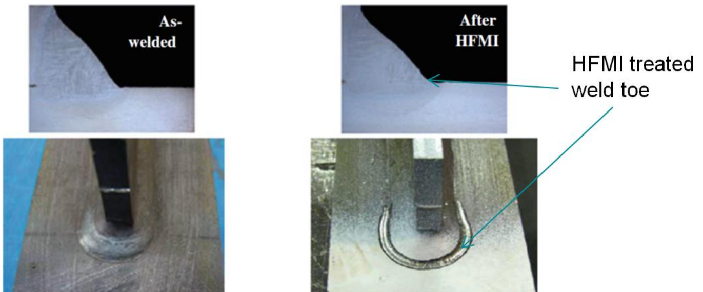
Figure 3. Typical application of post-weld treatment HFMI; Left: a MAG fillet weld in as-welded condition and Right: after HFMI treatment (from [1])
