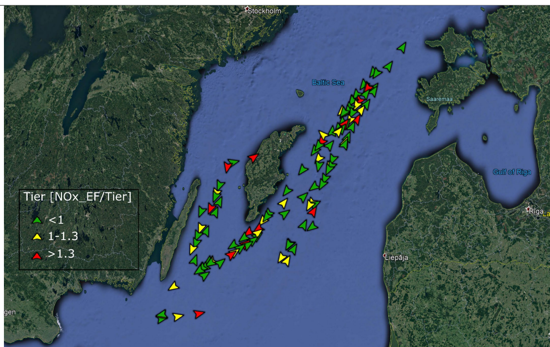
Figure 16. Airborne power specific \text{NO}_x emission rates ( \text{g/kWh} ) divided by the Tier I and Tier II limits for individual ships in the Baltic sea. Red means 30% above the limit.
