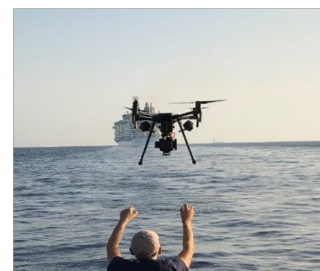
Denmark, Finland and Sweden, small drones with mini sniffers
