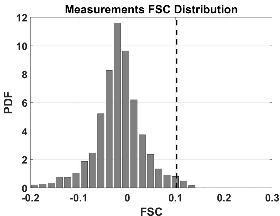
FIGURE 9. Statistical distribution (probability density function) of the measured FSC, corresponding to individual ships measured with sniffer at the Great Belt Bridge (3910 ships, medium and high quality). The dotted line is the estimated non-compliance limit for which the instrument errors (precision and bias) have been accounted for. The measured data set has a median and average FSC values of -0.018% and -0.0172 %, respectively. The standard deviation is 0.047 % and the 75 th and 90 th percentiles are 0.009% and 0.042 % in FSC units, respectively.
