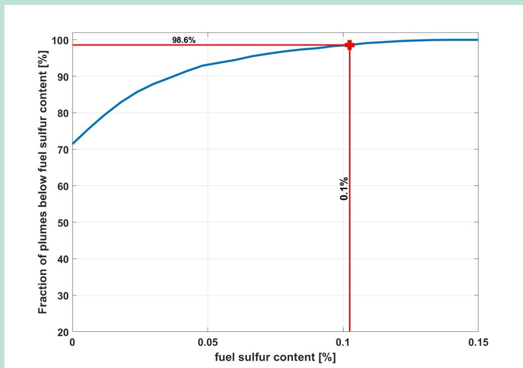
FIGURE 11. The fraction of ships that were measured below a certain FSC level at the Great Belt Bridge for the measurement period. In addition, the biased and noise corrected compliance limit threshold is shown.
