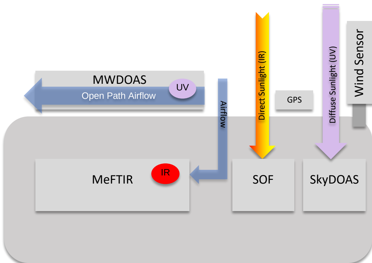
Figure 1. Overview of the mobile lab main instruments; SOF, MeFTIR, MWDOAS and SkyDOAS. SOF and SkyDOAS are column integrating passive techniques using the sun as the light source while MeFTIR and MWDOAS measure near ground-level concentrations using active internal light sources.
