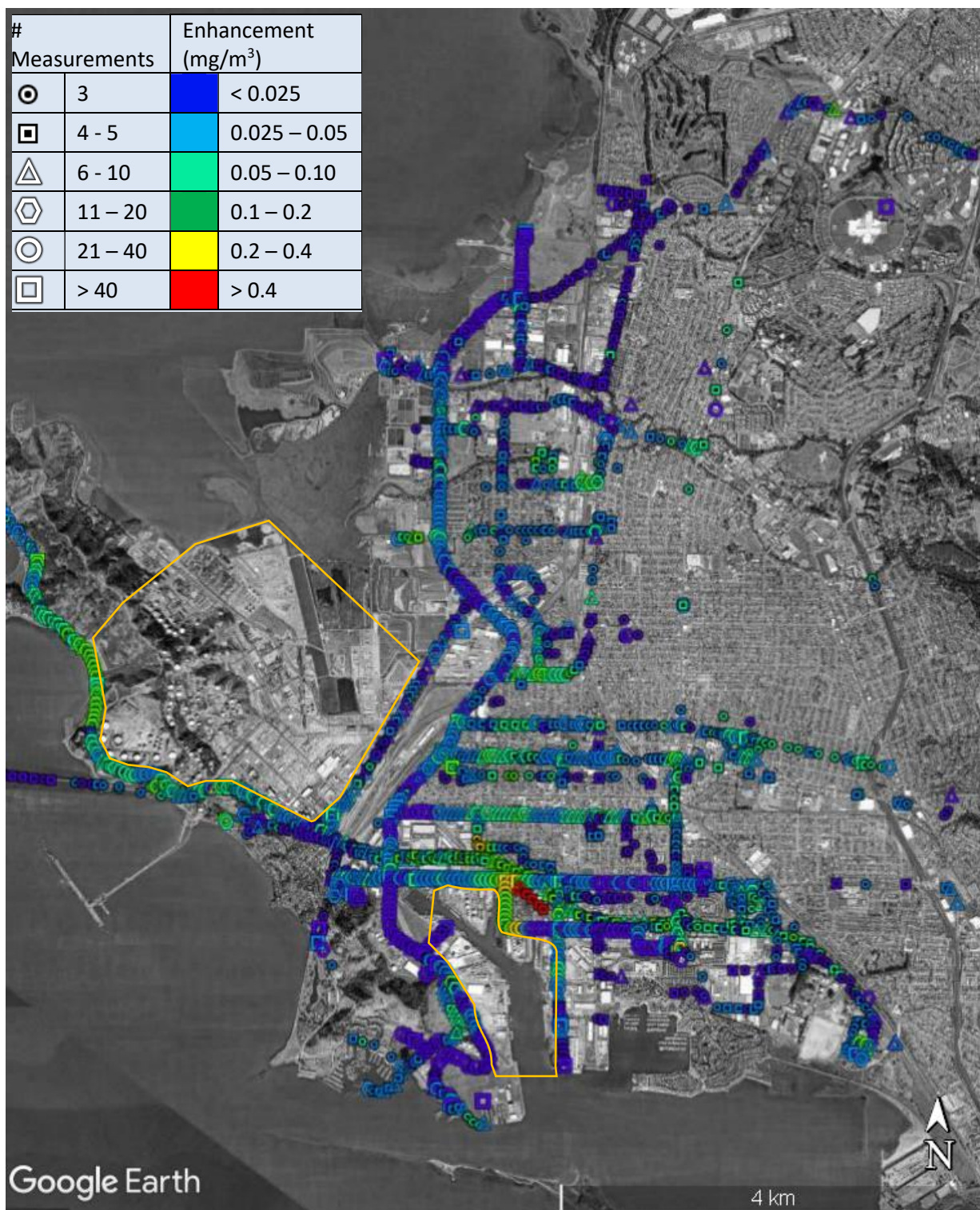
Figure 11. Concentration map of alkanes in Richmond for the Bay Area survey A, October 2018. Number of measurements (min. 3) within an approximately 50 x 50 m grid cell and mean alkane enhancement within the cell. Areas outlined in orange show approximate boundaries for the refinery (northwest) and port (south) areas. Map from Google Earth™, 2018.
