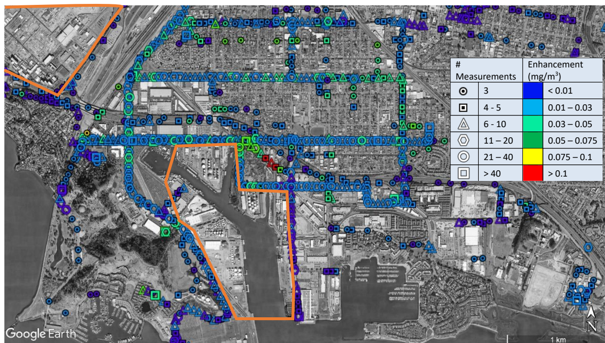
Figure E1. Concentration map of BTEX in Richmond (survey A), number of measurements (min. 3) within an approximately 50 x 50 m grid cell and mean BTEX enhancement within the cell. Oct, 2018. Highlighted areas show approximate boundaries for the refinery (northwest) and port (south) areas.
