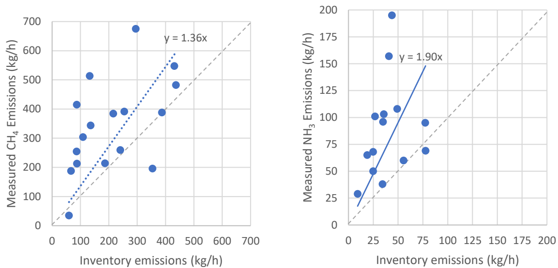
Figure 23. Relationship between measured and inventoried emissions, 1:1 and linear least squares fit plotted: (left) methane (right) ammonia.
