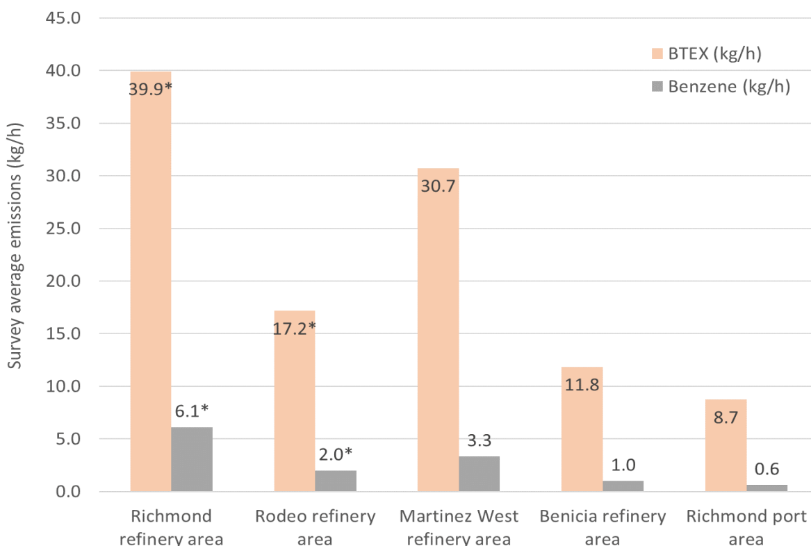
Figure 10. BTEX and benzene emissions for the Bay Area survey A measured indirectly from the ground-level ratio of BTEX (benzene, toluene, ethylbenzene and xylene) to alkanes and benzene to alkanes multiplied by the SOF alkane flux. *Limited number of samples.
