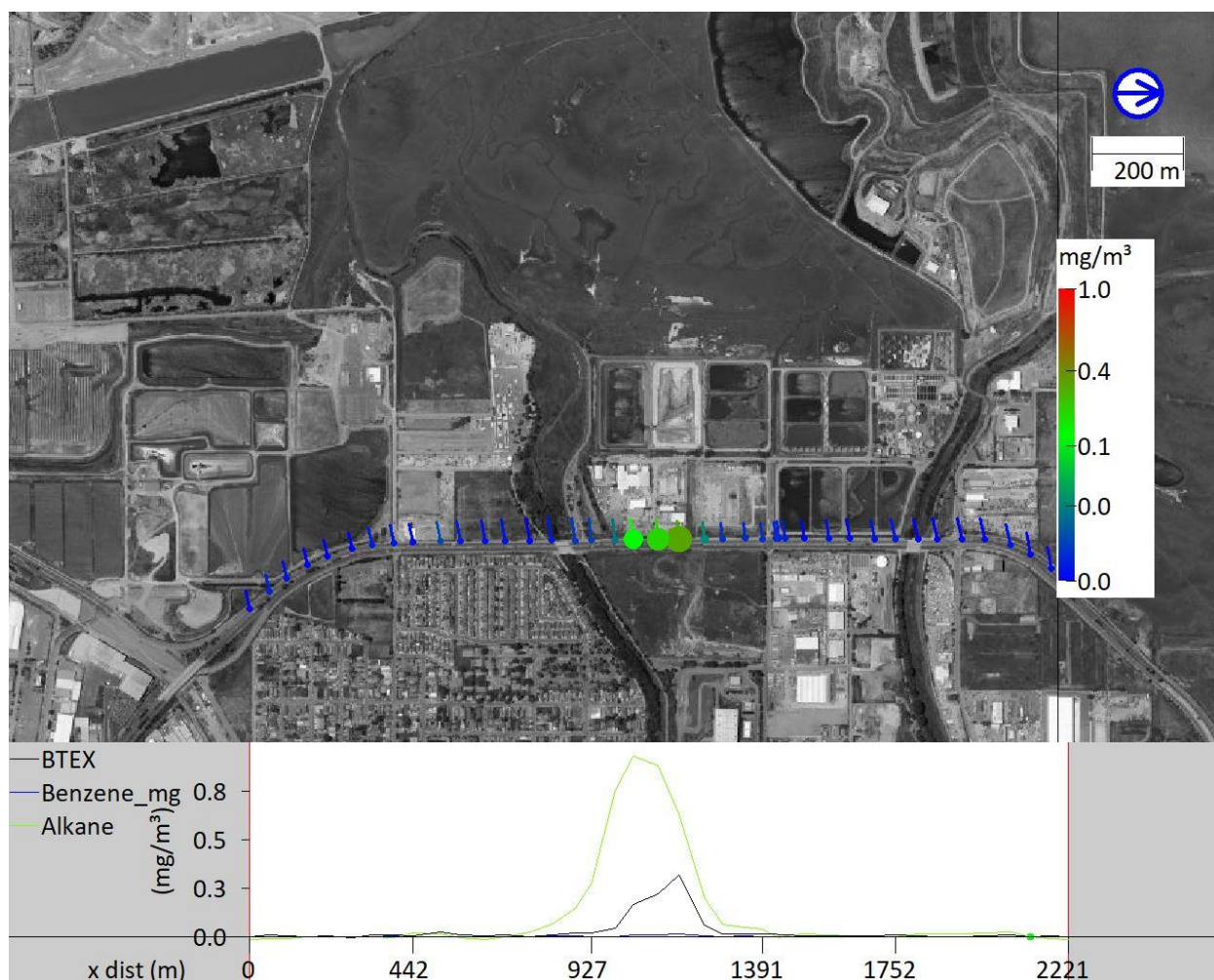
Figure 21. Temporary but unusually large VOC plume from the vicinity of the Pittsburg Ave intersection with Richmond Parkway (Survey A), Oct 23, 2018, 6PM. Image shows total BTEX in logarithmic color scale with lines point upwind in the direction of the source. The plot below the image shows BTEX ( 0.31 \text{ mg/m}^3 ), benzene, and alkane concentrations ( 1 \text{ mg/m}^3 ).
