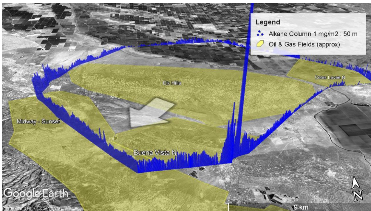
Figure 14. Alkane emission measurement around Elk Hills (survey B) with north-easterly winds, May 1, 2019, 13:35 – 15:14. SOF alkane column (apparent height of blue overlay) had a maximum of 341 mg/m 2 , near a source in Buena Vista. White arrow shows average wind direction during the measurement. Highlighted areas show approximate field boundaries for Elk Hills, Midway-Sunset, Coles Levee N and the northern portion of Buena Vista. Map from Google Earth™, 2021.
