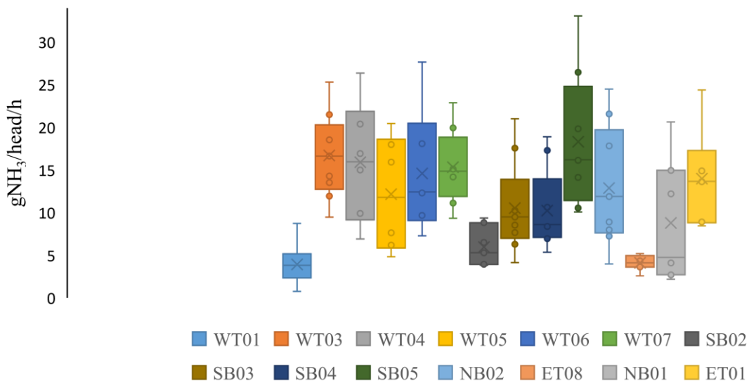
Figure 17. Ammonia emission factors obtained in the SJV dairy farm survey C. Displayed parameters: the minimum value, 25th percentile, median, mean, 75th percentile, maximum and individual values (filled circles).
