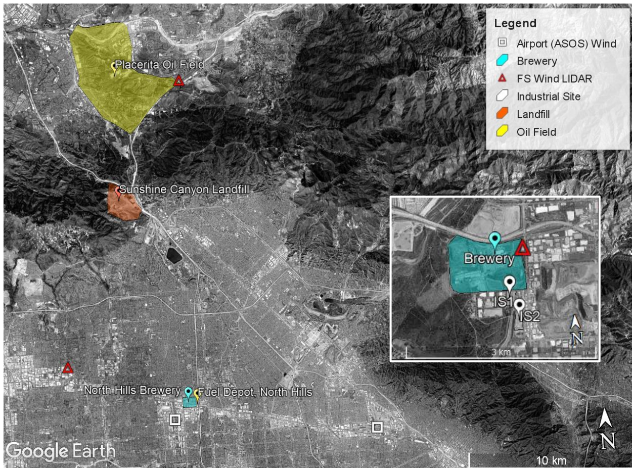
Figure 8. Measured areas in the north part of the South Coast Air Basin during survey D, Oct 2019. Inset Irwindale industrial sites (IS) and brewery. Map from Google Earth™, 2020.
