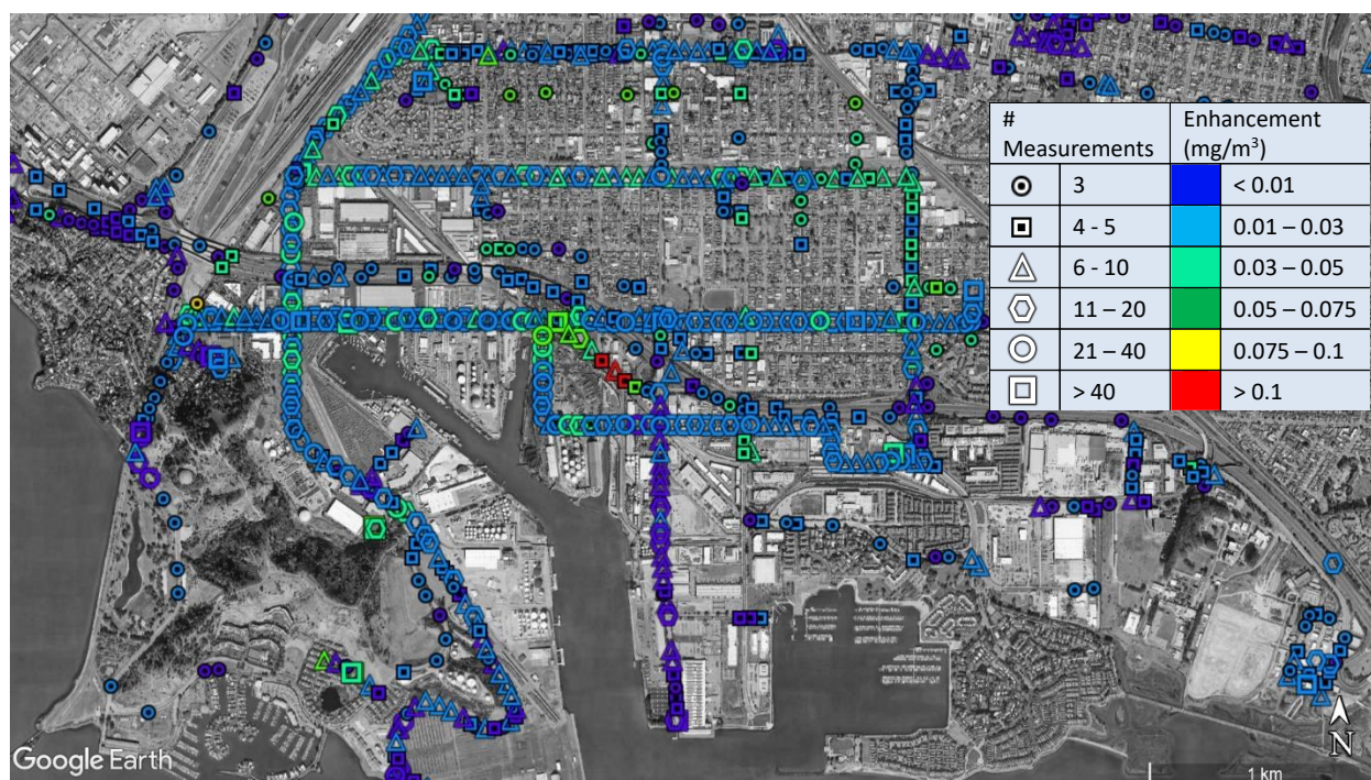
Figure 13. Concentration map of BTEX in Richmond (survey A), number of measurements (min. 3) within an approximately 50 x 50 m grid cell and mean BTEX enhancement within the cell. October 2018. Map from Google Earth™, 2018.
