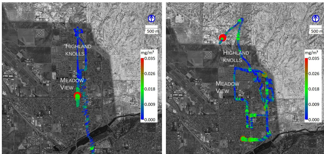
Figure 15. SJV BTEX concentration community monitoring measurements in the Bakersfield communities of Highland Knolls and Meadow View (survey B), May 2, 2019, 22:33 – 23:18 (Left) and 23:31 – May 3, 00:39 (Right). Color scale and point size show BTEX concentrations ( \text{mg}/\text{m}^3 ) and the lines point in the instantaneous wind direction.
