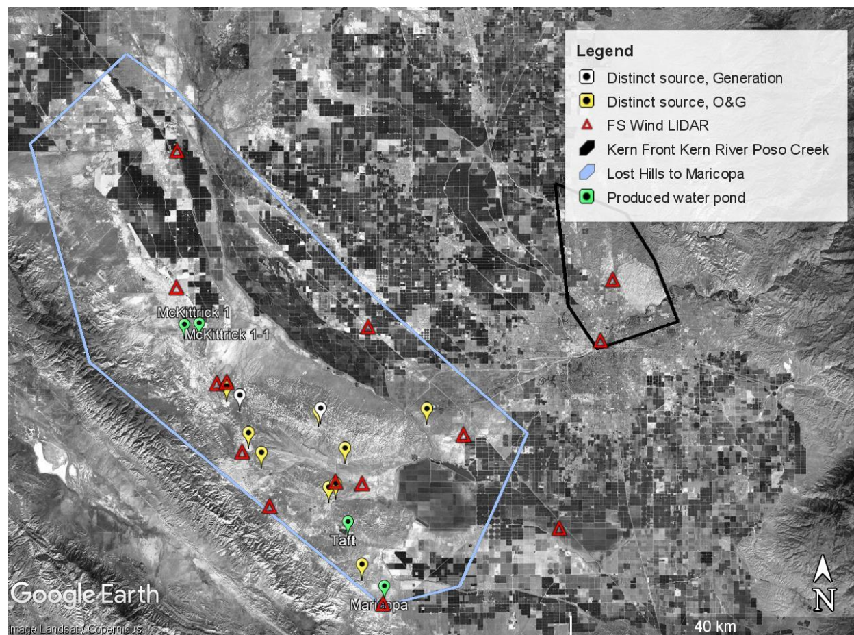
Figure 4. The primary oil and gas areas in the San Joaquin Valley that were studied in the emissions survey B during May 2019 and October 2018. The polygon to the left incorporates the fields of Lost Hills, Belridge, Cymric, McKittrick, Elk Hills, Midway-Sunset and Buena Vista. The polygon to the right incorporates Poso Creek, Kern Front, Kern River, Round Mountain and Mount Poso. In addition to the fields themselves, processing facilities and power generation facilities were also surveyed.
