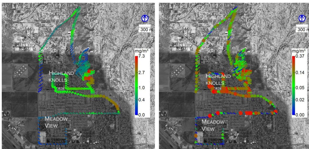
Figure 16. SJV methane and alkane concentration community monitoring measurements in the Bakersfield communities of Highland Knolls and Meadow View (survey B), May 17, 2019, 21:56 – 23:00. Color scale and point size show methane (left) and alkane (right) concentrations ( \text{mg}/\text{m}^3 ) and the lines point in the instantaneous wind direction. Color scale is logarithmic.
