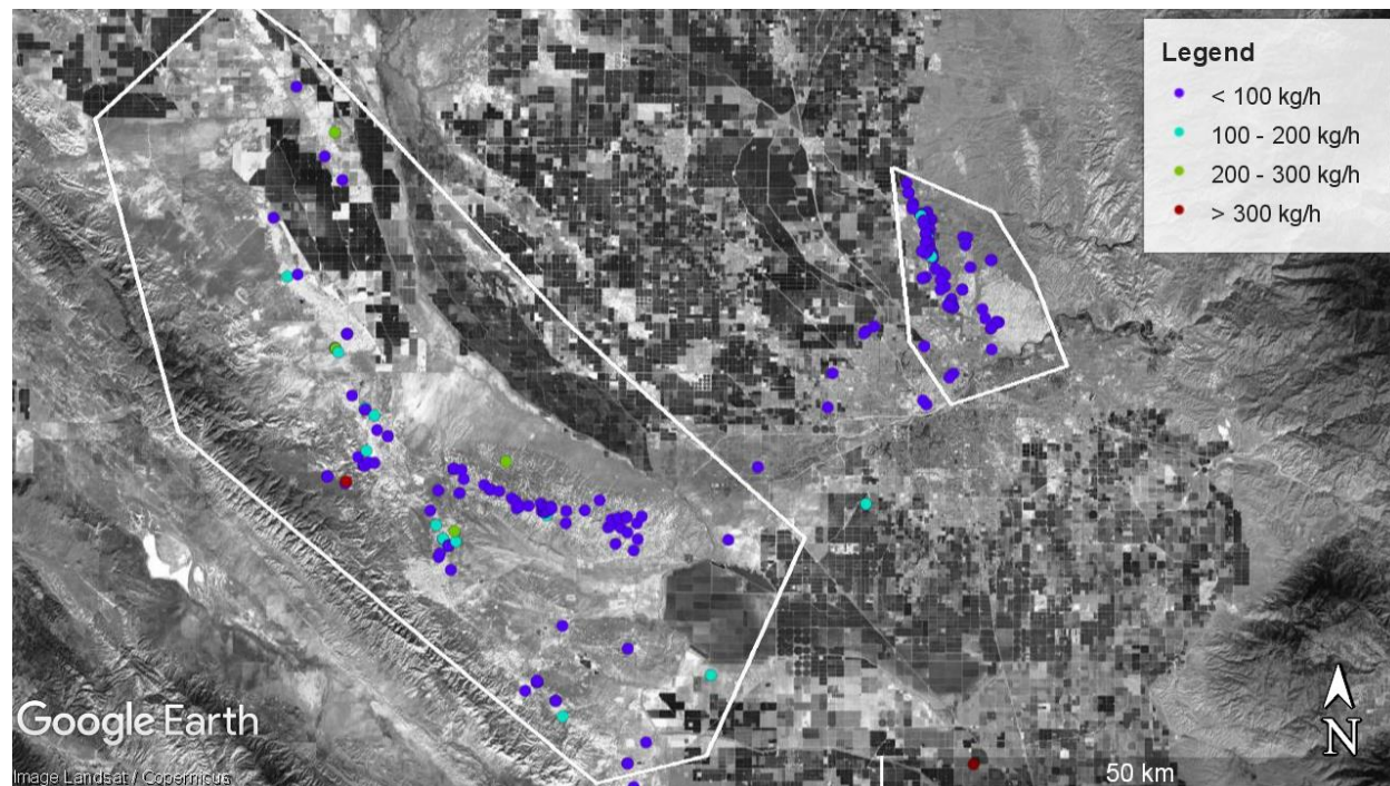
Figure 22. JPL measured methane plumes within the current survey area (B and C), colored by estimate emission. Source: Methane Source Finder ( https://methane.jpl.nasa.gov/ , Dec 13, 2019).
