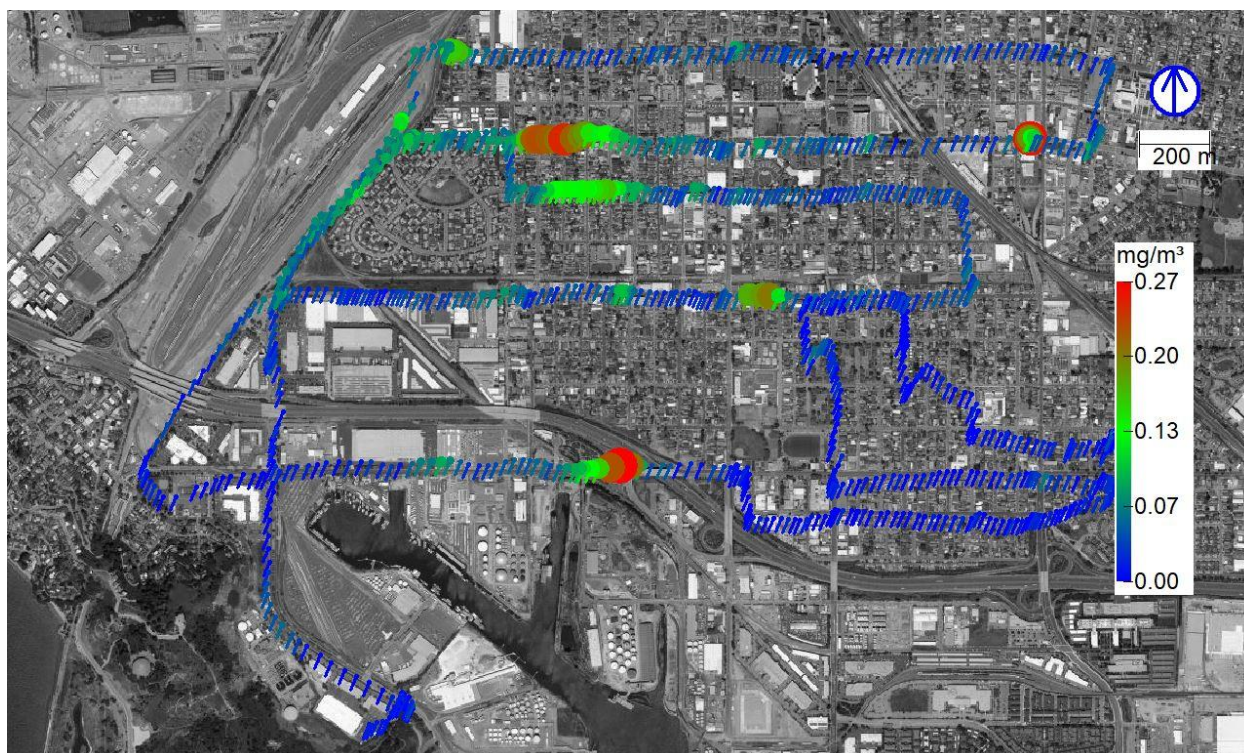
Figure 12. Tracking the VOC (alkane) plume from the Port of Richmond into the Richmond community using MeFTIR (survey A). Marker size and color show concentration with a line point in the upwind direction toward the source. Daytime measurement. October 20, 2018.
