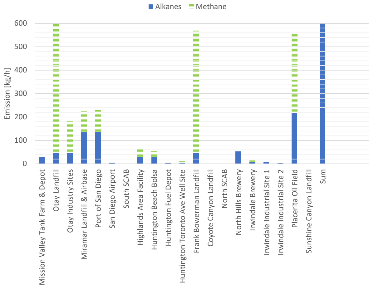
Figure 18. Median values of VOC emissions (alkanes and methane) from the sites during survey D 2019 as measured by the SOF, MWDOAS and MeFTIR instruments. Alkane emissions are measured directly while methane emissions are indirectly measured (IME) from gas ratios.
