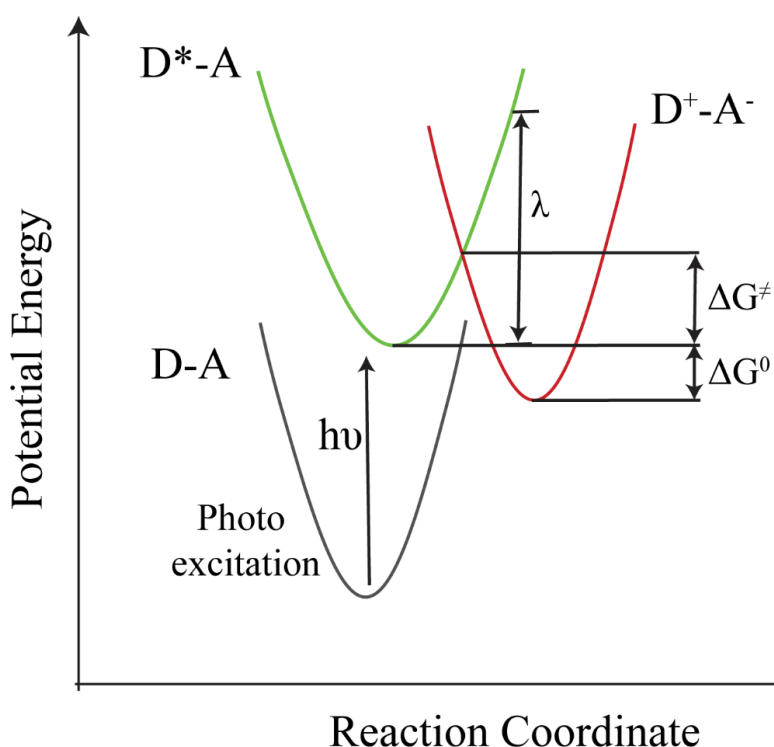
Figure 2.4. Potential energy surface diagram showing PET from photoexcitation of a donor. The diagram includes the ground state ( D-A ), the initially photoexcited state ( D^*-A ) and the charge separated state ( D^+-A^- ). The driving force ( \Delta G^0 ), activation energy ( \Delta G^\ddagger ) and reorganization energy ( \lambda ) are also indicated in the diagram.
