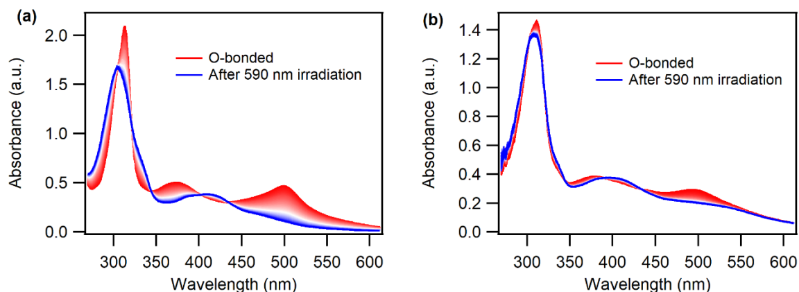
Figure 5.3. Absorption changes of O\text{-[Ru(deeb)}_2\text{PySO-iPr)]}^{2+} over time (from red to blue spectra) following continuous irradiation with 590 nm light in (a) DCM liquid solution and (b) attached to a \text{ZrO}_2 thin film ( \sim 50 \text{ nmol/cm}^2 ) in air. Reproduced with permission from Paper II 133 .
