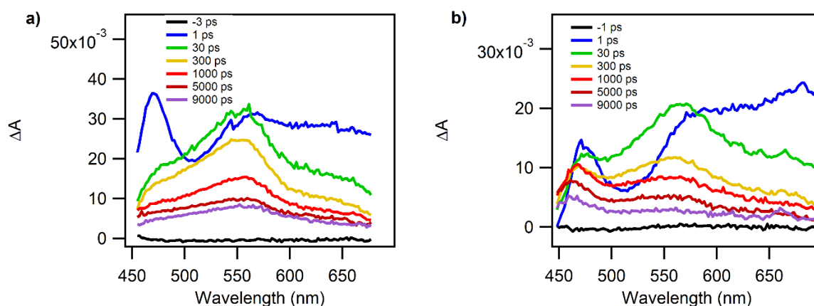
Figure 4.5. fs-TA spectra of DPIBFC6/SnO 2 in (a) acetonitrile and (b) toluene. Reproduced with permission from Paper I 118 .
