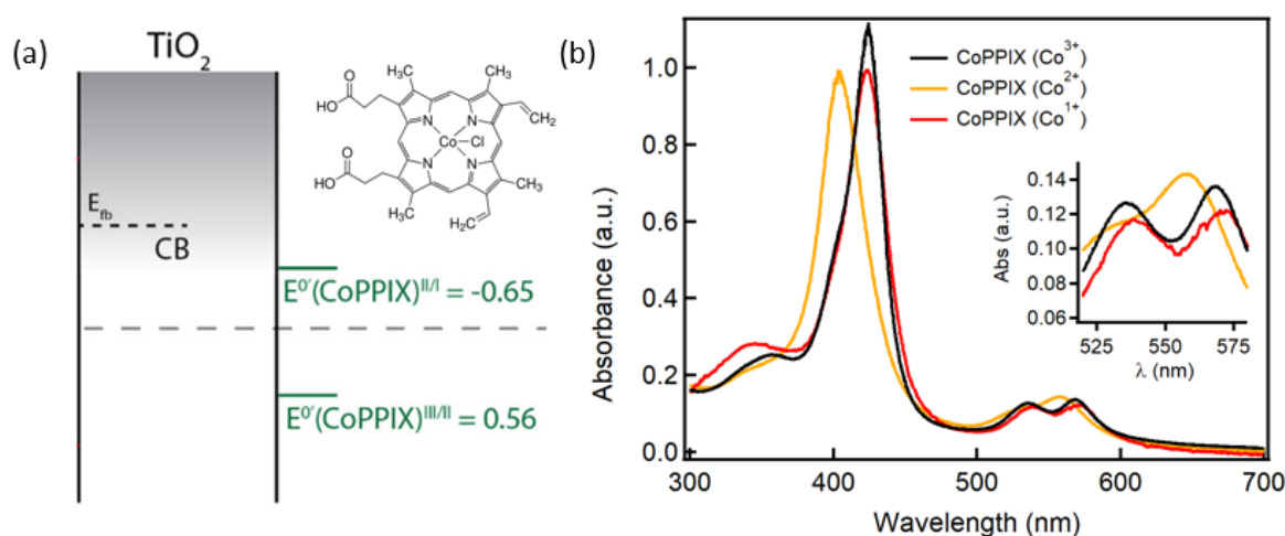
Figure 3.7. (a) Molecular structure and redox potentials for one- and two-electron reduction of CoPPIX (vs NHE) in relation to the CB energy level of \text{TiO}_2 , where the dotted line represents the zero-line vs NHE (b) Absorption spectra of the different redox states of CoPPIX. Adapted with permission from Paper IV 173 . Copyright 2018 American Chemical Society.
