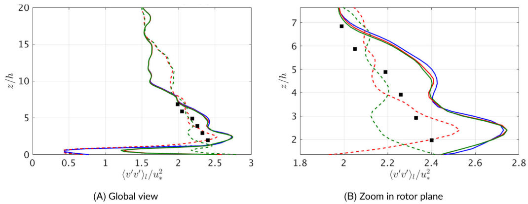
FIGURE 14 (A,B) \langle v'v' \rangle_1 / u_*^2 at the location of the wind turbine. —: Wind Turbine 1 in homogeneous forest, - - : Wind Turbine 2 in homogeneous forest, —: Wind Turbine 1 in current clearing, - - : Wind Turbine 2 in current clearing, —: Wind Turbine 1 in extended clearing, - - : Wind Turbine 2 in extended clearing, ■: measurements (no data for error bars available) 33,34
