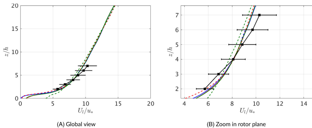
FIGURE 10 (A,B) \langle U_i/u_* \rangle at the location of the wind turbines. —: Wind Turbine 1 in homogeneous forest, - - -: Wind Turbine 2 in homogeneous forest, —: Wind Turbine 1 in current clearing, - - -: Wind Turbine 2 in current clearing, —: Wind Turbine 1 in extended clearing, - - -: Wind Turbine 2 in extended clearing, —■—: measurements 33,34
