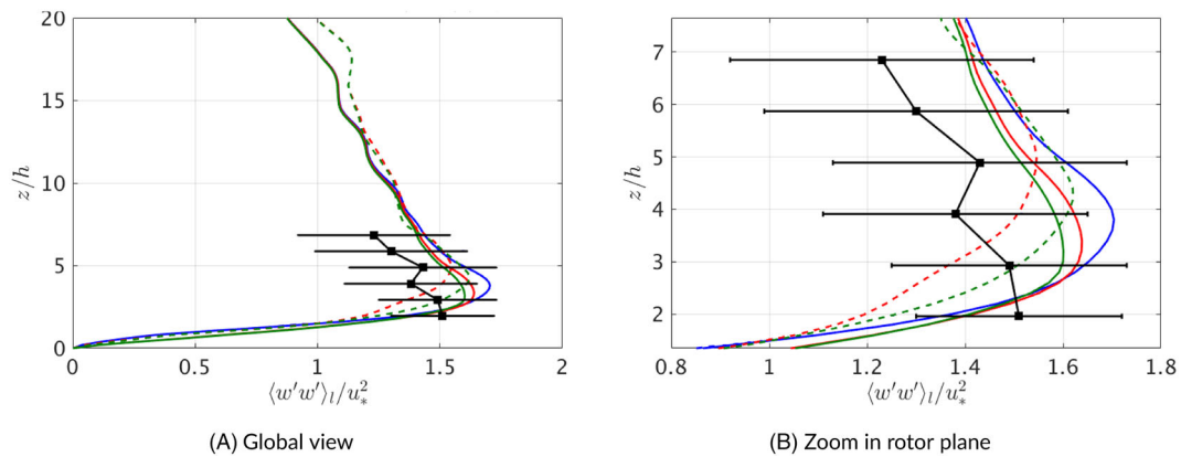
FIGURE 15 (A,B) \langle w'w' \rangle_1 / u_*^2 at the location of the wind turbine. —: Wind Turbine 1 in homogeneous forest, - - : Wind Turbine 2 in homogeneous forest, —: Wind Turbine 1 in current clearing, - - : Wind Turbine 2 in current clearing, —: Wind Turbine 1 in extended clearing, - - : Wind Turbine 2 in extended clearing, ■: measurements 33,34
