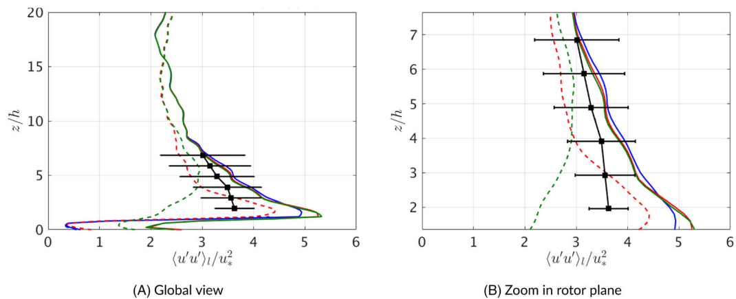
FIGURE 13 (A,B) \langle u'u' \rangle_1 / u_*^2 at the location of the wind turbine. —: Wind Turbine 1 in homogeneous forest, - - : Wind Turbine 2 in homogeneous forest, —: Wind Turbine 1 in current clearing, - - : Wind turbine 2 in current clearing, —: Wind Turbine 1 in extended clearing, - - : Wind Turbine 2 in extended clearing, —■: measurements 33,34
