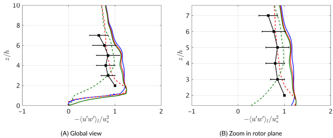
FIGURE 12 (A,B) -\langle u'w' \rangle_1 / u_*^2 at the location of the wind turbine. —: Wind Turbine 1 in homogeneous forest, - - : Wind Turbine 2 in homogeneous forest, —: Wind Turbine 1 in current clearing, - - : Wind Turbine 2 in current clearing, —: Wind Turbine 1 in extended clearing, - - : Wind Turbine 2 in extended clearing, —■: measurements 33,34
