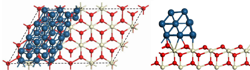
Figure 5.14: Pt rod supported on \text{CeO}_2(111) . Left: top view. Right: side view.
